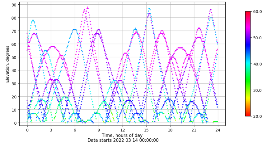
Time-elevation plot for station SALA. Signal to Noise S1C Data file SALA00ESP_R_2022073.xtr
