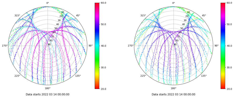
Skyplot for station SALA. Signal to Noise S1C Data file SALA00ESP_R_2022073.xtr Skyplot for station SALA. Signal to Noise S2P Data file SALA00ESP_R_2022073.xtr
