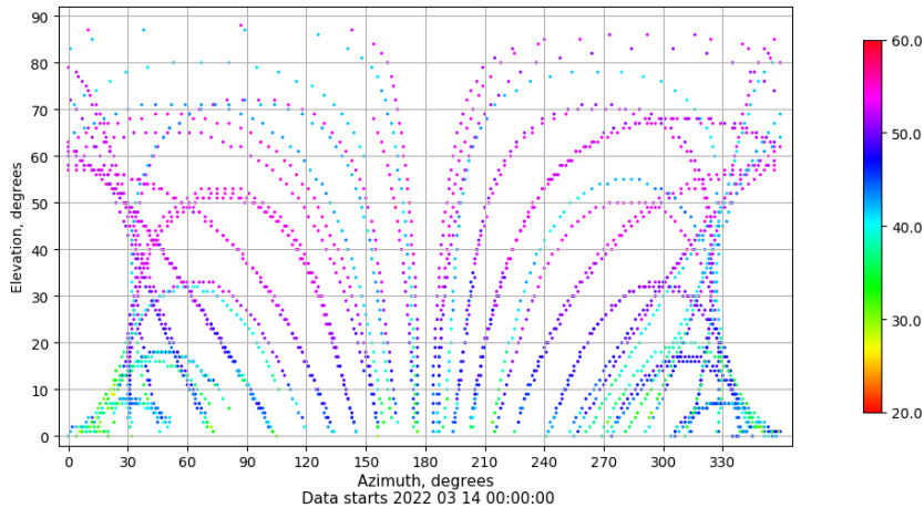
Azimuth-elevation plot for station SALA. Signal to Noise S1C Data file SALA00ESP_R_2022073.xtr
