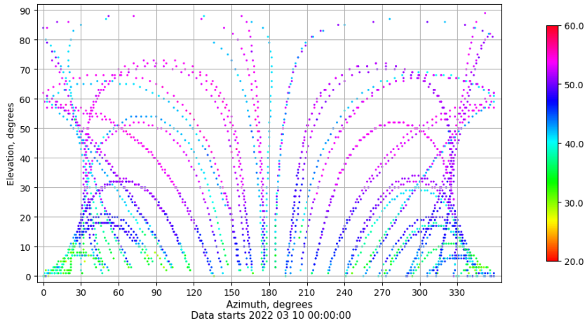
Azimuth-elevation plot for station SALA. Signal to Noise S1C Data file SALA00ESP_R_2022069.xtr
