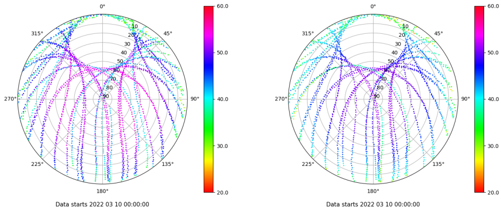
Skyplot for station SALA. Signal to Noise S1C Data file SALA00ESP_R_2022069.xtr Skyplot for station SALA. Signal to Noise S2P Data file SALA00ESP_R_2022069.xtr
