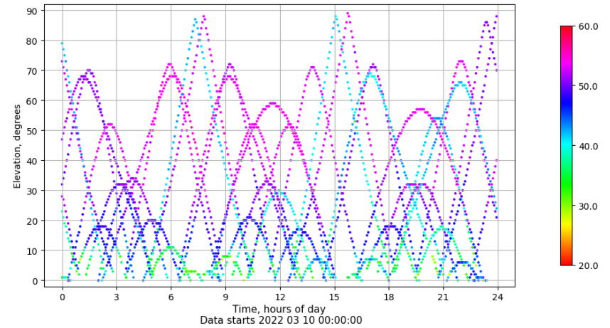
Time-elevation plot for station SALA. Signal to Noise S1C Data file SALA00ESP_R_2022069.xtr
