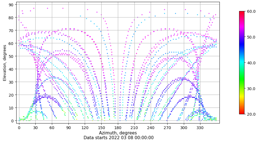
Azimuth-elevation plot for station SALA. Signal to Noise S1C Data file SALA00ESP_R_2022067.xtr
