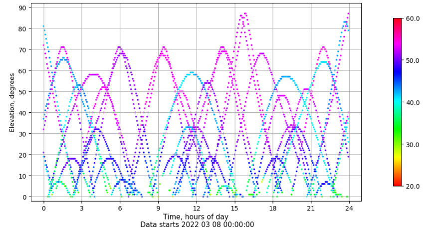
Time-elevation plot for station SALA. Signal to Noise S1C Data file SALA00ESP_R_2022067.xtr
