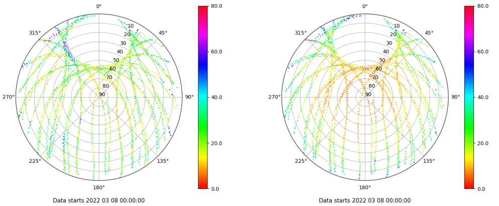
Skyplot for station SALA. Parameter M1C Data file SALA00ESP_R_2022067.xtr Skyplot for station SALA. Parameter M2P Data file SALA00ESP_R_2022067.xtr
