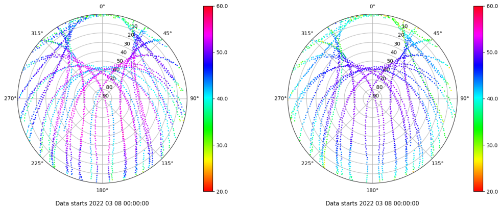
Skyplot for station SALA. Signal to Noise S1C Data file SALA00ESP_R_2022067.xtr Skyplot for station SALA. Signal to Noise S2P Data file SALA00ESP_R_2022067.xtr
