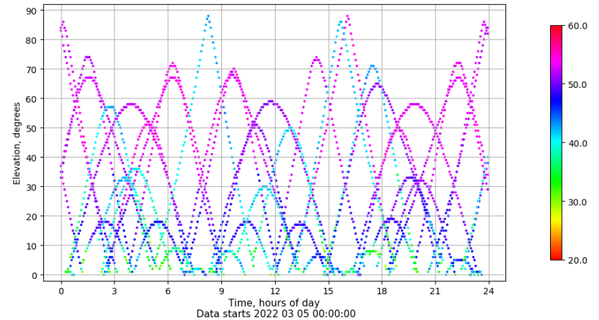
Time-elevation plot for station SALA. Signal to Noise S1C Data file SALA00ESP_R_2022064.xtr
