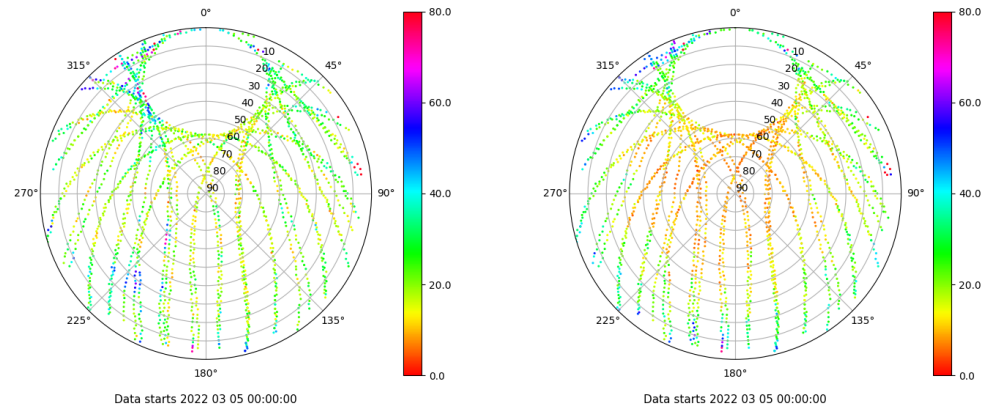
Skyplot for station SALA. Parameter M1C Data file SALA00ESP_R_2022064.xtr Skyplot for station SALA. Parameter M2P Data file SALA00ESP_R_2022064.xtr
