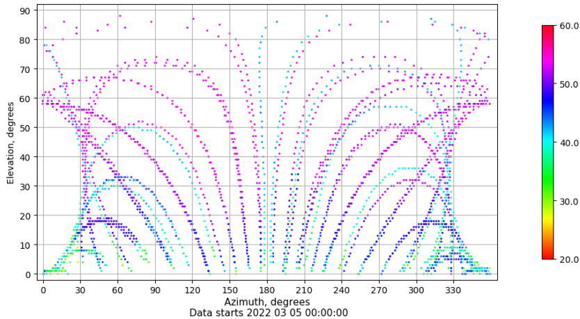
Azimuth-elevation plot for station SALA. Signal to Noise S1C Data file SALA00ESP_R_2022064.xtr
