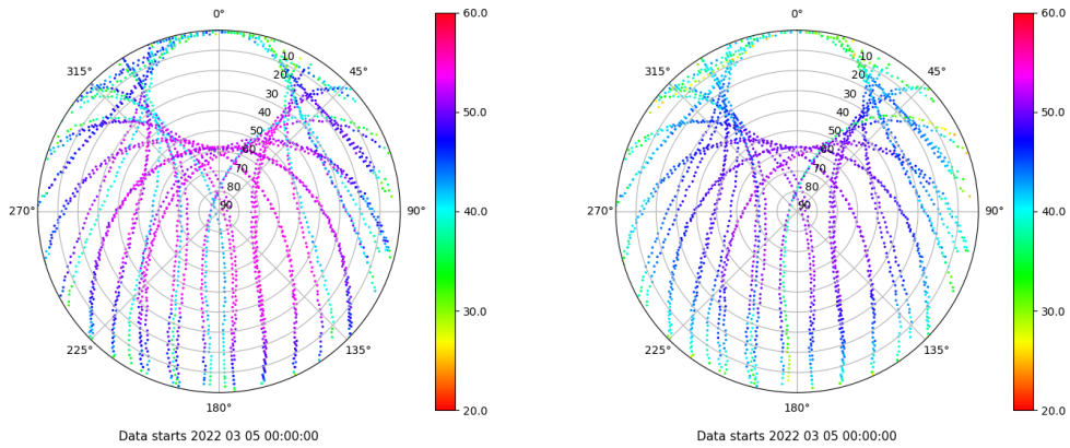
Skyplot for station SALA. Signal to Noise S1C Data file SALA00ESP_R_2022064.xtr Skyplot for station SALA. Signal to Noise S2P Data file SALA00ESP_R_2022064.xtr
