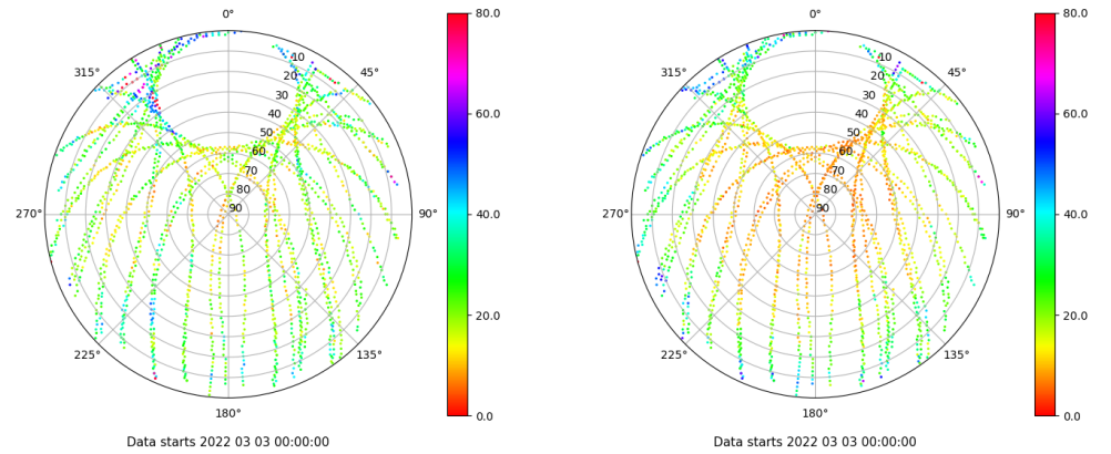
Skyplot for station SALA. Parameter M1C Data file SALA00ESP_R_2022062.xtr Skyplot for station SALA. Parameter M2P Data file SALA00ESP_R_2022062.xtr
