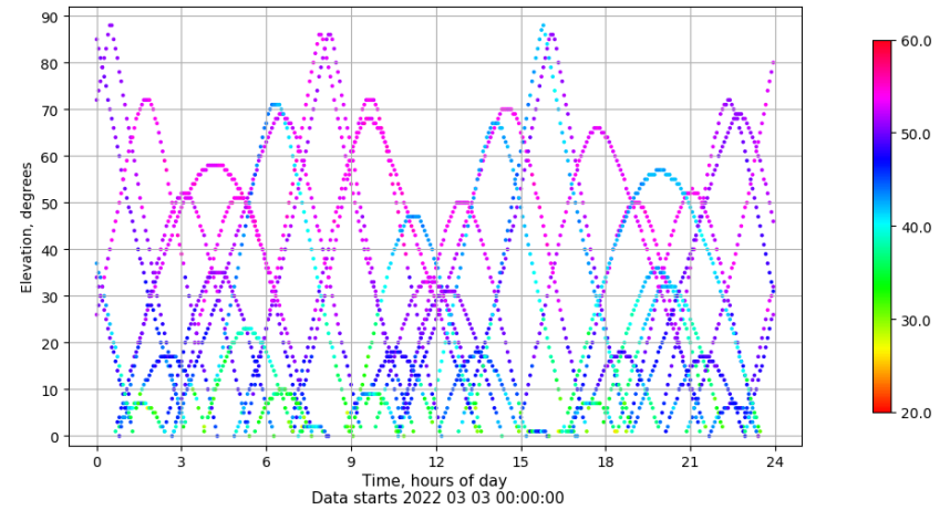
Time-elevation plot for station SALA. Signal to Noise S1C Data file SALA00ESP_R_2022062.xtr
