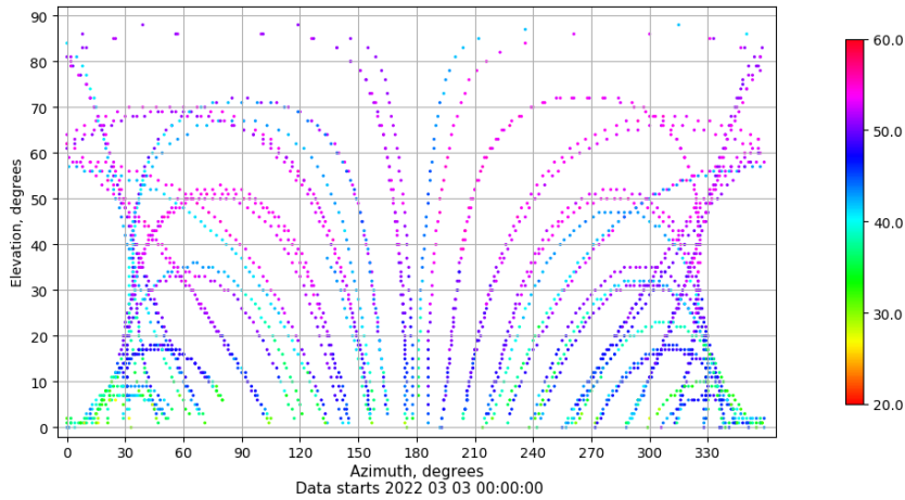
Azimuth-elevation plot for station SALA. Signal to Noise S1C Data file SALA00ESP_R_2022062.xtr
