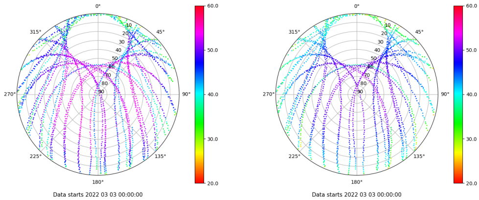
Skyplot for station SALA. Signal to Noise S1C Data file SALA00ESP_R_2022062.xtr Skyplot for station SALA. Signal to Noise S2P Data file SALA00ESP_R_2022062.xtr
