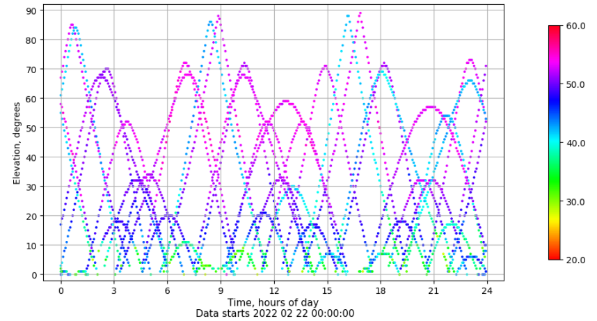
Time-elevation plot for station SALA. Signal to Noise S1C Data file SALA00ESP_R_2022053.xtr
