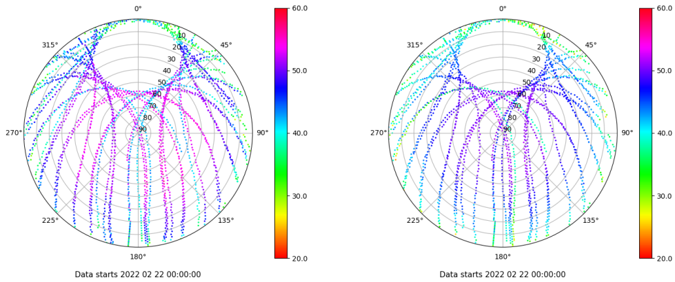
Skyplot for station SALA. Signal to Noise S1C Data file SALA00ESP_R_2022053.xtr Skyplot for station SALA. Signal to Noise S2P Data file SALA00ESP_R_2022053.xtr
