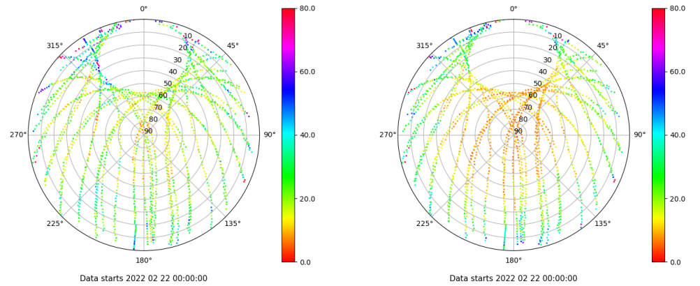
Skyplot for station SALA. Parameter M1C Data file SALA00ESP_R_2022053.xtr Skyplot for station SALA. Parameter M2P Data file SALA00ESP_R_2022053.xtr
