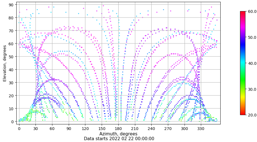
Azimuth-elevation plot for station SALA. Signal to Noise S1C Data file SALA00ESP_R_2022053.xtr
