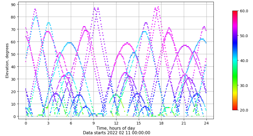
Time-elevation plot for station SALA. Signal to Noise S1C Data file SALA00ESP_R_2022042.xtr
