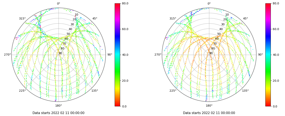
Skyplot for station SALA. Parameter M1C Data file SALA00ESP_R_2022042.xtr Skyplot for station SALA. Parameter M2P Data file SALA00ESP_R_2022042.xtr
