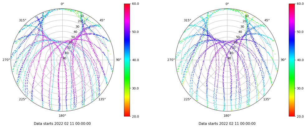
Skyplot for station SALA. Signal to Noise S1C Data file SALA00ESP_R_2022042.xtr Skyplot for station SALA. Signal to Noise S2P Data file SALA00ESP_R_2022042.xtr
