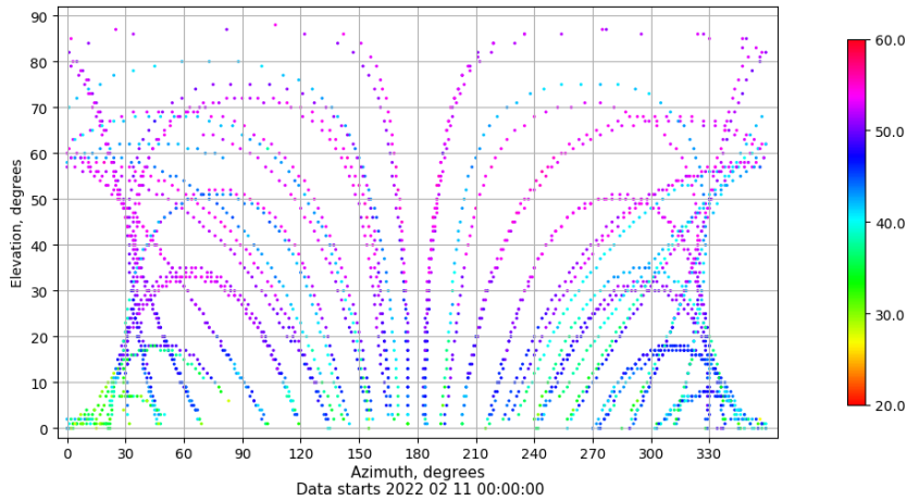
Azimuth-elevation plot for station SALA. Signal to Noise S1C Data file SALA00ESP_R_2022042.xtr
