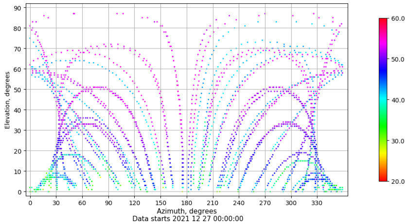
Azimuth-elevation plot for station SALA. Signal to Noise S1C Data file SALA00ESP_R_2021361.xtr
