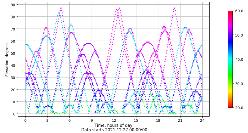
Time-elevation plot for station SALA. Signal to Noise S1C Data file SALA00ESP_R_2021361.xtr
