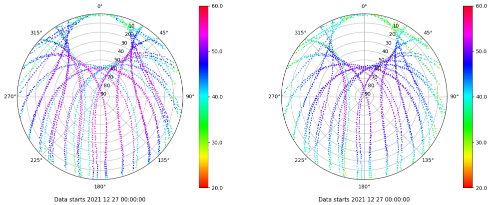
Skyplot for station SALA. Signal to Noise S1C Data file SALA00ESP_R_2021361.xtr Skyplot for station SALA. Signal to Noise S2P Data file SALA00ESP_R_2021361.xtr
