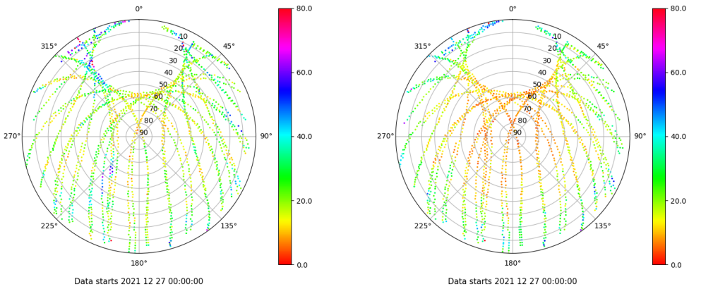
Skyplot for station SALA. Parameter M1C Data file SALA00ESP_R_2021361.xtr Skyplot for station SALA. Parameter M2P Data file SALA00ESP_R_2021361.xtr
