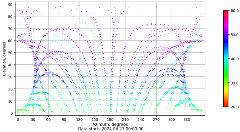
Azimuth-elevation plot for station RODI. Signal to Noise S1C Data file RODI00ESP_R_2024118.xtr
