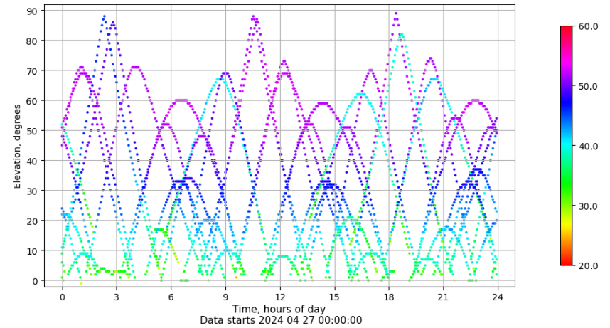
Time-elevation plot for station RODI. Signal to Noise S1C Data file RODI00ESP_R_2024118.xtr
