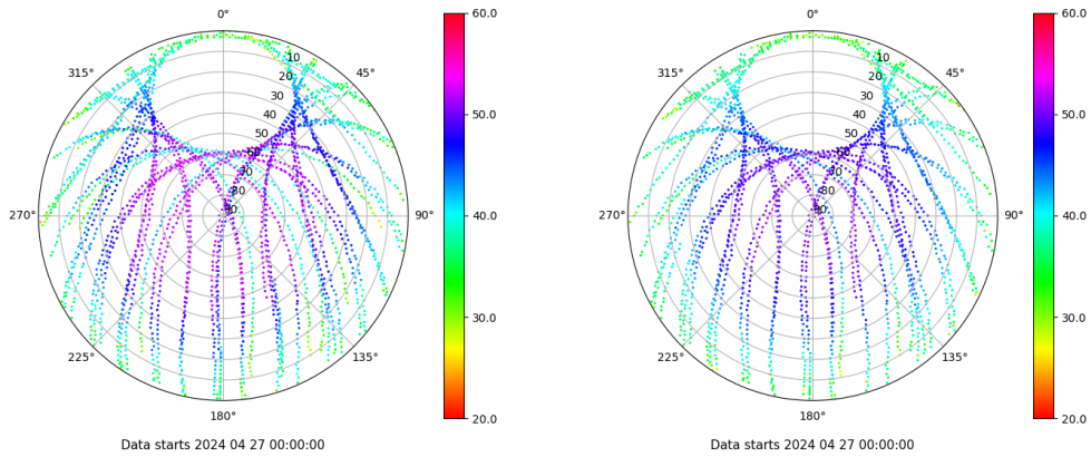
Skyplot for station RODI. Signal to Noise S1C Data file RODI00ESP_R_2024118.xtr Skyplot for station RODI. Signal to Noise S2C Data file RODI00ESP_R_2024118.xtr
