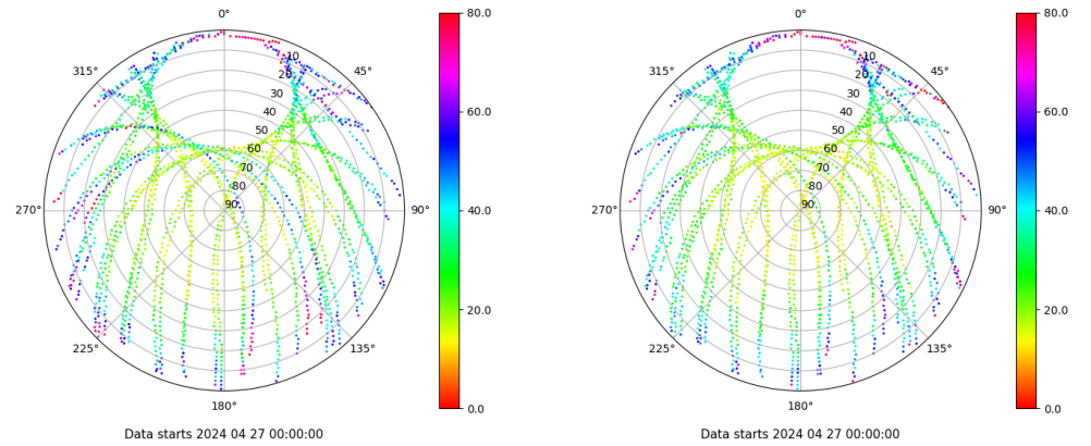
Skyplot for station RODI. Parameter M1C Data file RODI00ESP_R_2024118.xtr Skyplot for station RODI. Parameter M2C Data file RODI00ESP_R_2024118.xtr
