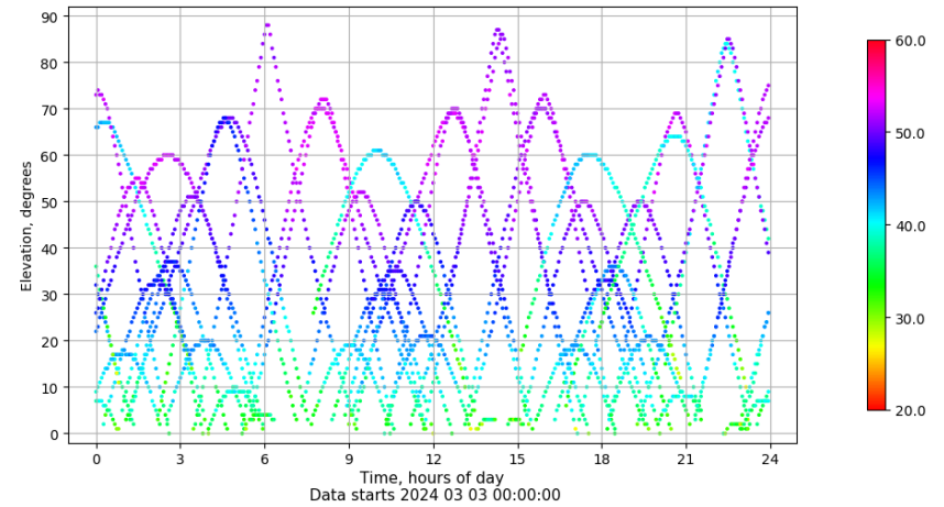
Time-elevation plot for station RODI. Signal to Noise S1C Data file RODI00ESP_R_2024063.xtr
