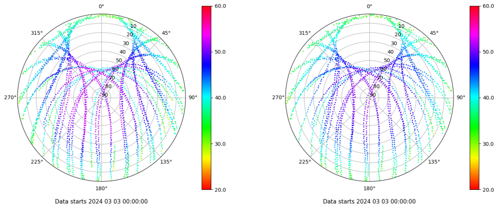
Skyplot for station RODI. Signal to Noise S1C Data file RODI00ESP_R_2024063.xtr Skyplot for station RODI. Signal to Noise S2C Data file RODI00ESP_R_2024063.xtr
