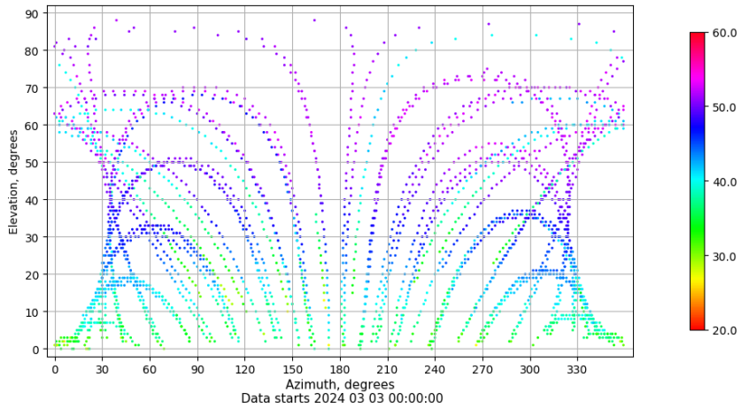
Azimuth-elevation plot for station RODI. Signal to Noise S1C Data file RODI00ESP_R_2024063.xtr
