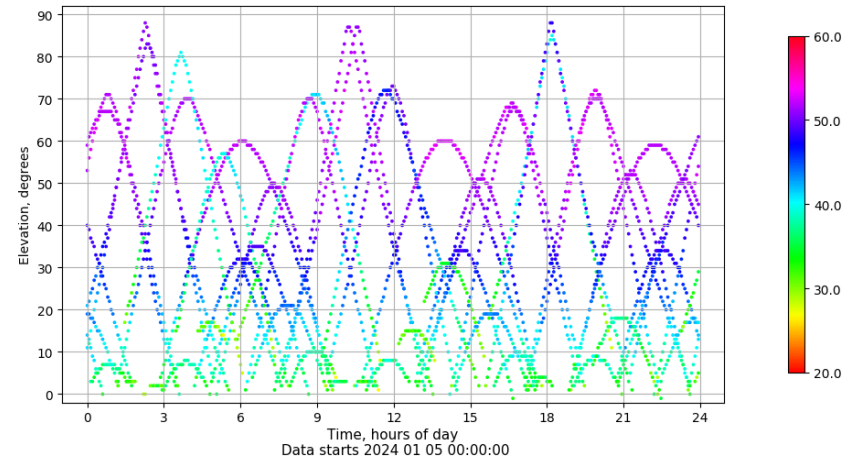
Time-elevation plot for station RODI. Signal to Noise S1C Data file RODI00ESP_R_2024005.xtr
