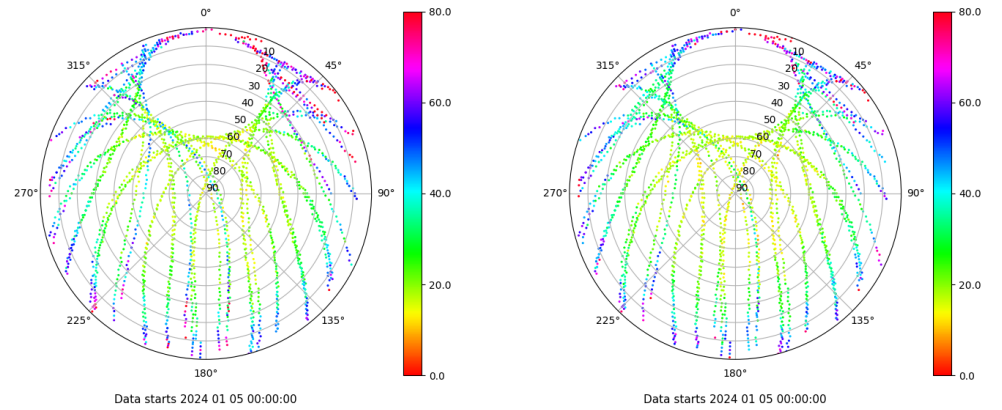
Skyplot for station RODI. Parameter M1C Data file RODI00ESP_R_2024005.xtr Skyplot for station RODI. Parameter M2C Data file RODI00ESP_R_2024005.xtr
