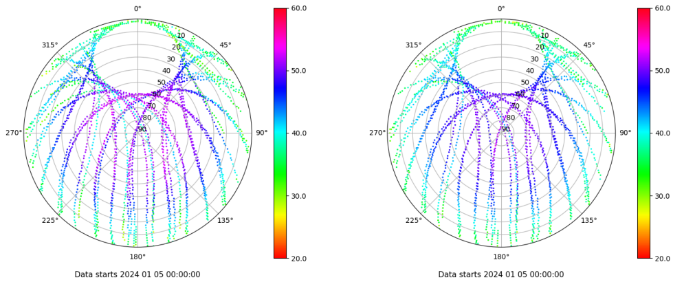
Skyplot for station RODI. Signal to Noise S1C Data file RODI00ESP_R_2024005.xtr Skyplot for station RODI. Signal to Noise S2C Data file RODI00ESP_R_2024005.xtr
