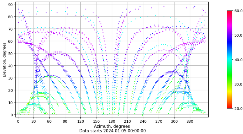
Azimuth-elevation plot for station RODI. Signal to Noise S1C Data file RODI00ESP_R_2024005.xtr
