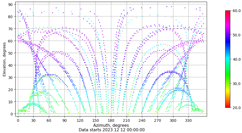
Azimuth-elevation plot for station RODI. Signal to Noise S1C Data file RODI00ESP_R_2023346.xtr
