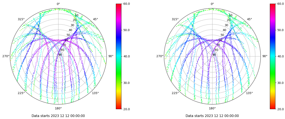
Skyplot for station RODI. Signal to Noise S1C Data file RODI00ESP_R_2023346.xtr Skyplot for station RODI. Signal to Noise S2C Data file RODI00ESP_R_2023346.xtr
