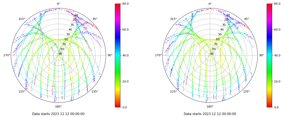
Skyplot for station RODI. Parameter M1C Data file RODI00ESP_R_2023346.xtr Skyplot for station RODI. Parameter M2C Data file RODI00ESP_R_2023346.xtr
