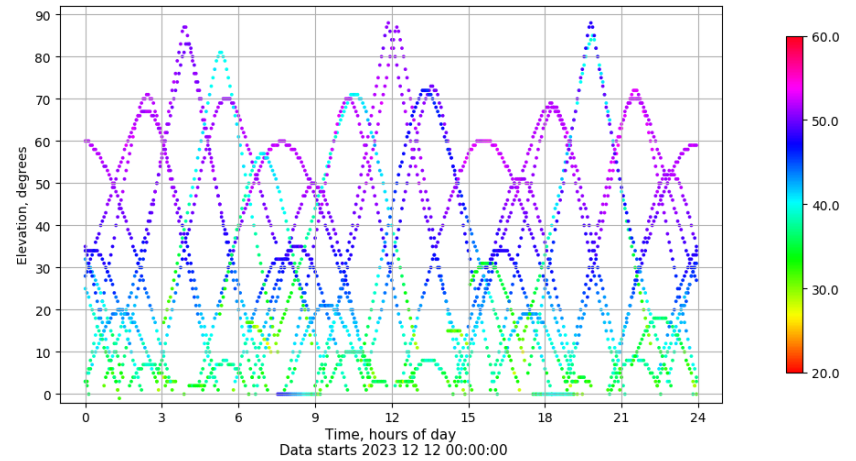
Time-elevation plot for station RODI. Signal to Noise S1C Data file RODI00ESP_R_2023346.xtr
