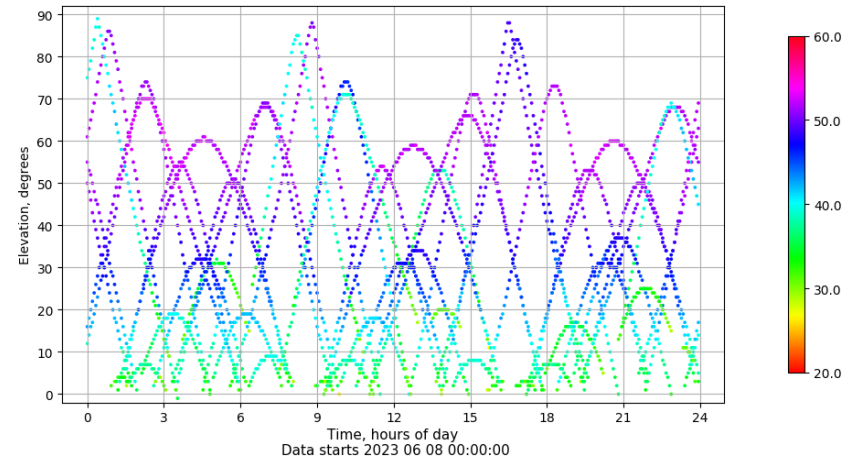
Time-elevation plot for station RODI. Signal to Noise S1C Data file RODI00ESP_R_2023159.xtr
