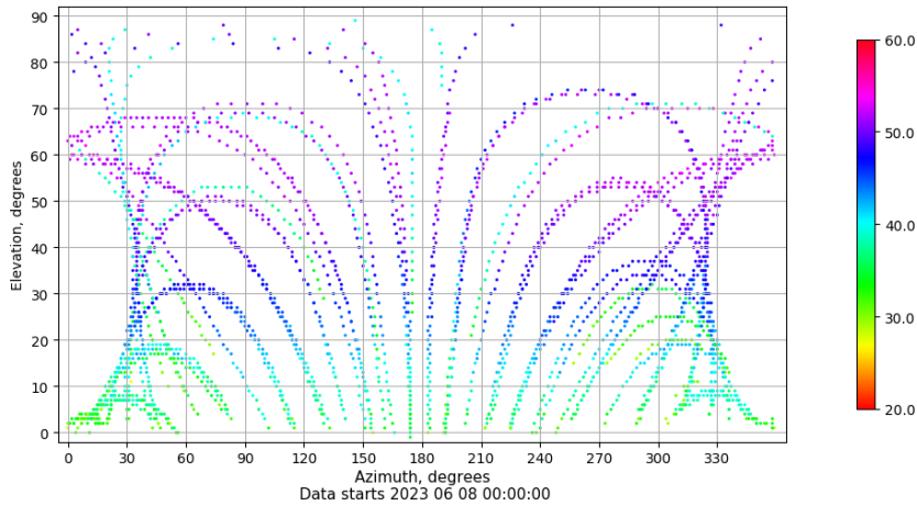
Azimuth-elevation plot for station RODI. Signal to Noise S1C Data file RODI00ESP_R_2023159.xtr
