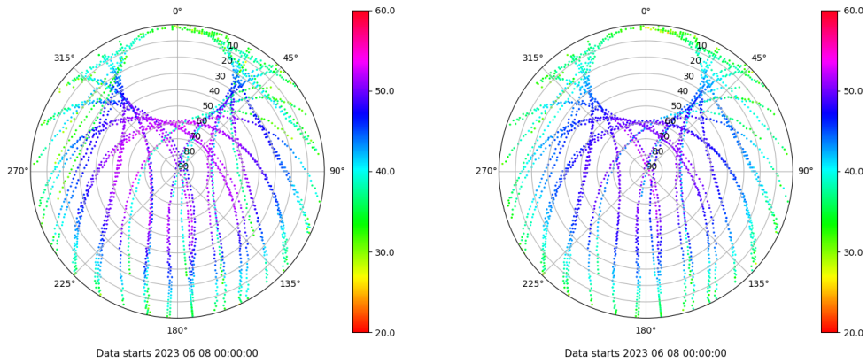
Skyplot for station RODI. Signal to Noise S1C Data file RODI00ESP_R_2023159.xtr Skyplot for station RODI. Signal to Noise S2C Data file RODI00ESP_R_2023159.xtr
