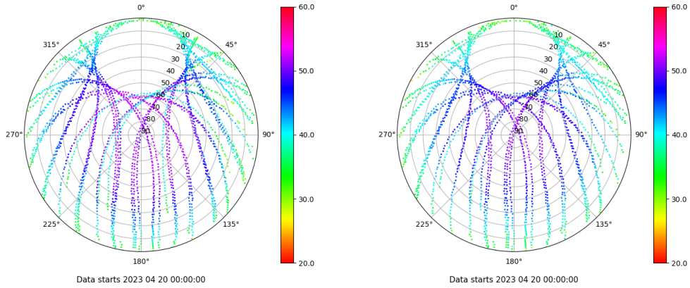
Skyplot for station RODI. Signal to Noise S1C Data file RODI00ESP_R_2023110.xtr Skyplot for station RODI. Signal to Noise S2C Data file RODI00ESP_R_2023110.xtr
