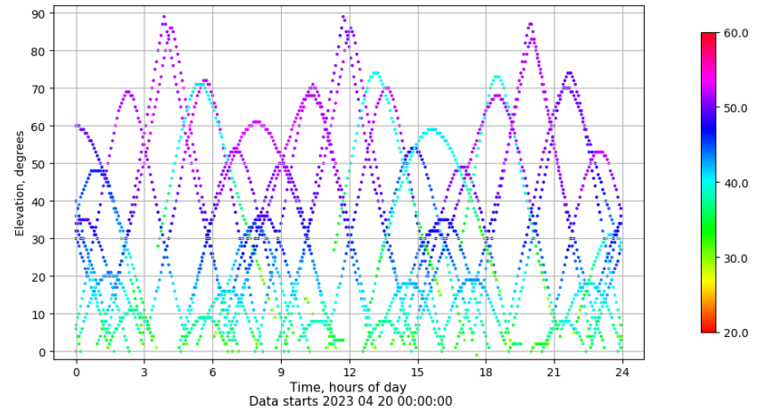
Time-elevation plot for station RODI. Signal to Noise S1C Data file RODI00ESP_R_2023110.xtr
