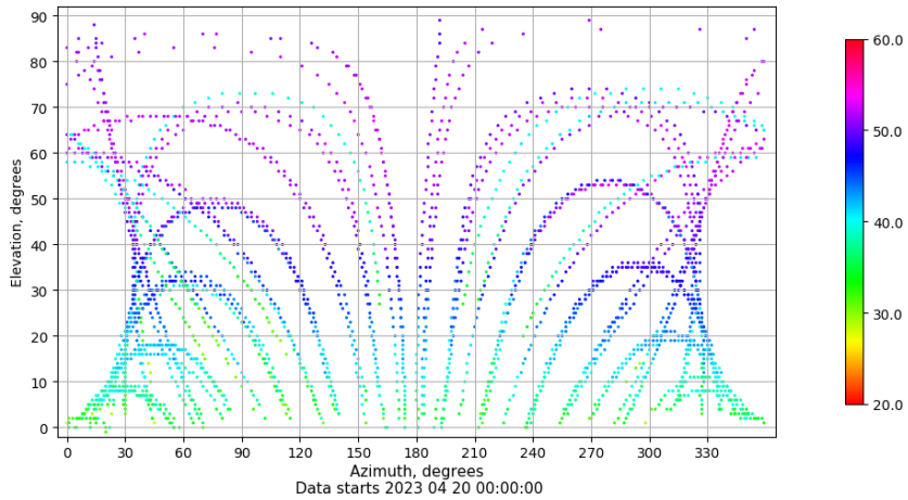
Azimuth-elevation plot for station RODI. Signal to Noise S1C Data file RODI00ESP_R_2023110.xtr
