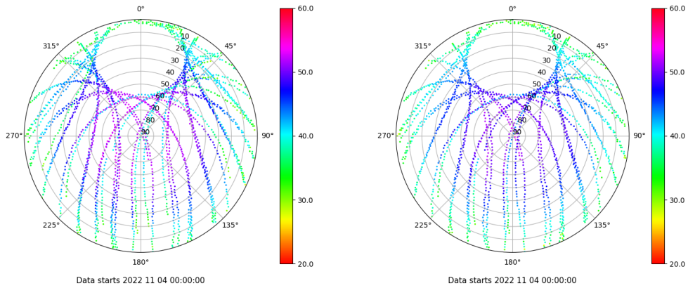
Skyplot for station RODI. Signal to Noise S1C Data file RODI00ESP_R_2022308.xtr Skyplot for station RODI. Signal to Noise S2C Data file RODI00ESP_R_2022308.xtr
