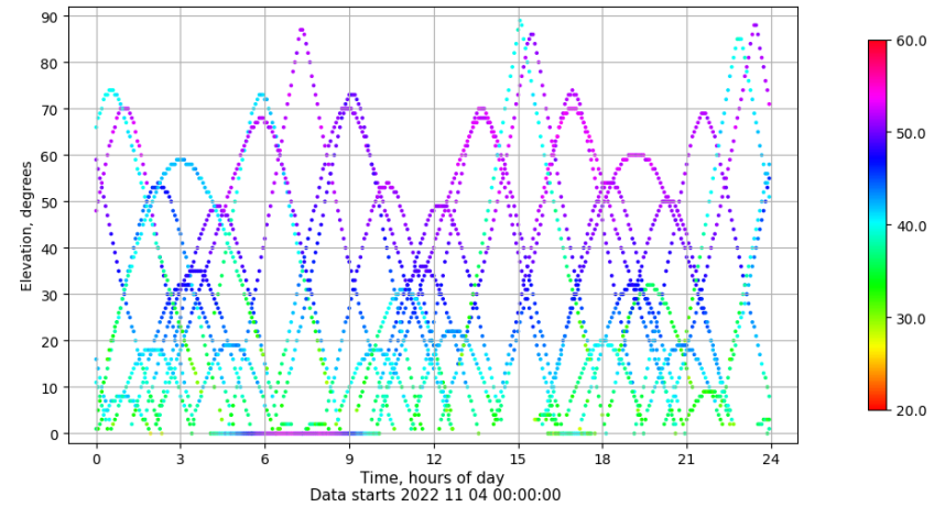
Time-elevation plot for station RODI. Signal to Noise S1C Data file RODI00ESP_R_2022308.xtr
