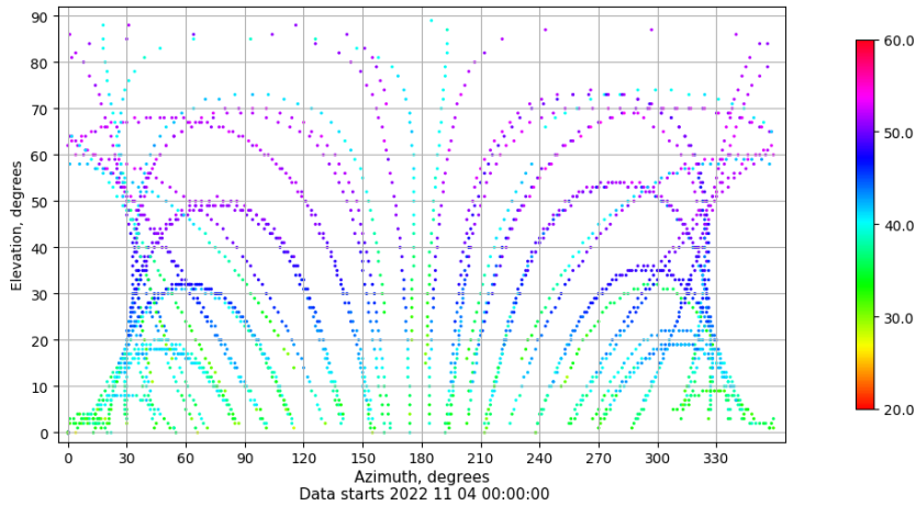
Azimuth-elevation plot for station RODI. Signal to Noise S1C Data file RODI00ESP_R_2022308.xtr
