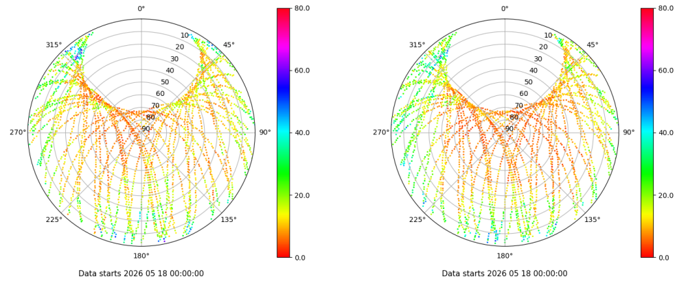
Skyplot for station RIO1. Parameter M1C Data file RIO100ESP_R_2026138.xtr Skyplot for station RIO1. Parameter M2W Data file RIO100ESP_R_2026138.xtr
