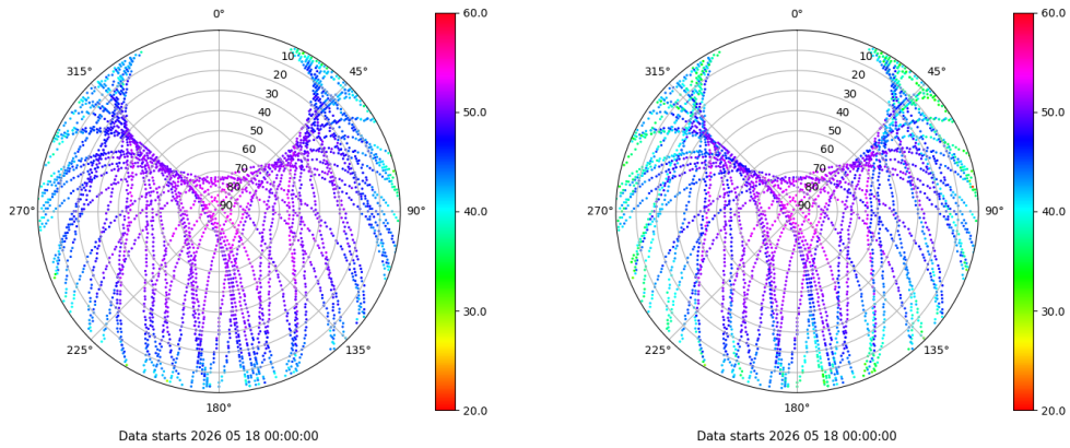
Skyplot for station RIO1. Signal to Noise S1C Data file RIO100ESP_R_2026138.xtr Skyplot for station RIO1. Signal to Noise S2W Data file RIO100ESP_R_2026138.xtr
