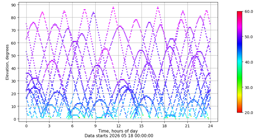
Time-elevation plot for station RIO1. Signal to Noise S1C Data file RIO100ESP_R_2026138.xtr
