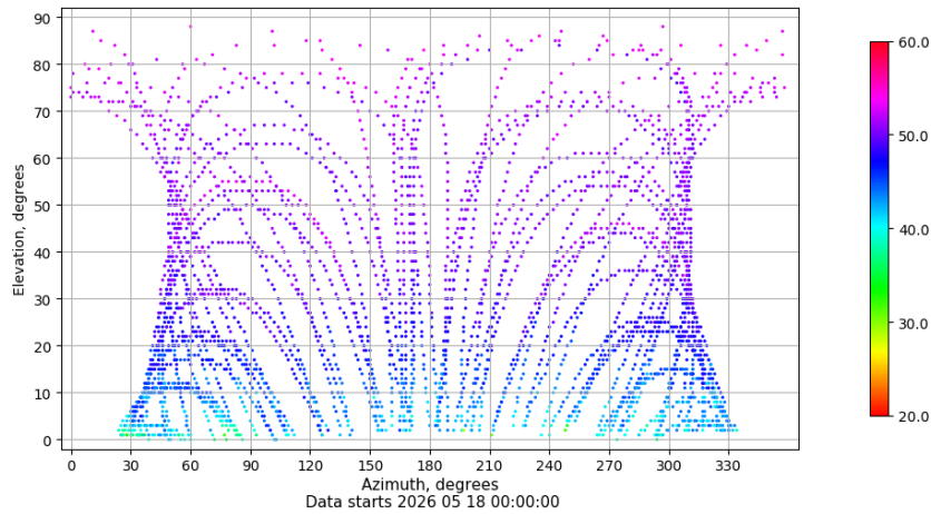
Azimuth-elevation plot for station RIO1. Signal to Noise S1C Data file RIO100ESP_R_2026138.xtr
