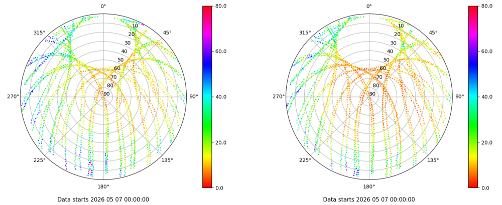
Skyplot for station RIO1. Parameter M1C Data file RIO100ESP_R_2026127.xtr Skyplot for station RIO1. Parameter M2P Data file RIO100ESP_R_2026127.xtr
