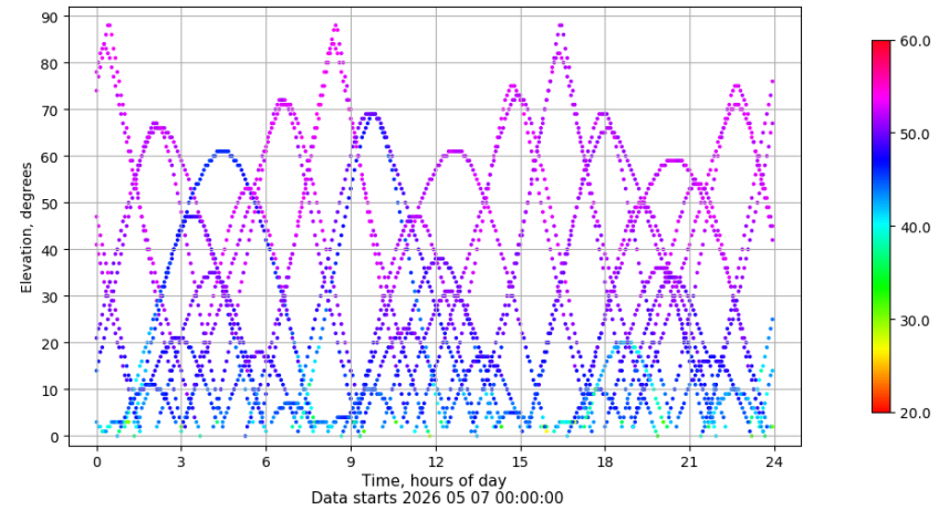
Time-elevation plot for station RIO1. Signal to Noise S1C Data file RIO100ESP_R_2026127.xtr
