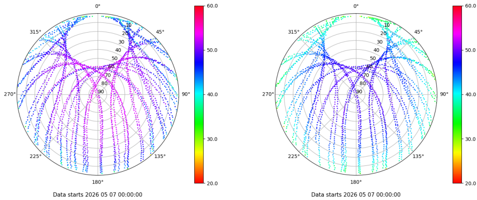
Skyplot for station RIO1. Signal to Noise S1C Data file RIO100ESP_R_2026127.xtr Skyplot for station RIO1. Signal to Noise S2P Data file RIO100ESP_R_2026127.xtr
