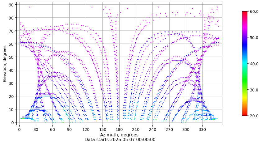
Azimuth-elevation plot for station RIO1. Signal to Noise S1C Data file RIO100ESP_R_2026127.xtr
