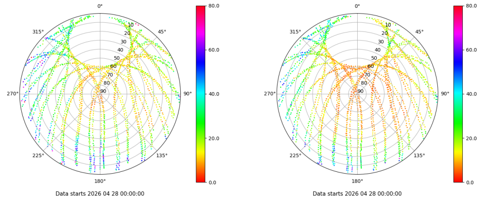
Skyplot for station RIO1. Parameter M1C Data file RIO100ESP_R_2026118.xtr Skyplot for station RIO1. Parameter M2P Data file RIO100ESP_R_2026118.xtr
