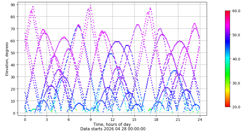
Time-elevation plot for station RIO1. Signal to Noise S1C Data file RIO100ESP_R_2026118.xtr
