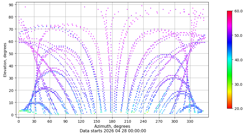
Azimuth-elevation plot for station RIO1. Signal to Noise S1C Data file RIO100ESP_R_2026118.xtr
