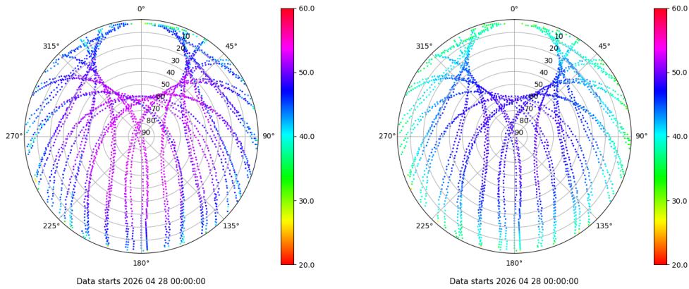
Skyplot for station RIO1. Signal to Noise S1C Data file RIO100ESP_R_2026118.xtr Skyplot for station RIO1. Signal to Noise S2P Data file RIO100ESP_R_2026118.xtr
