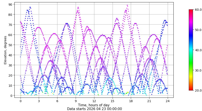
Time-elevation plot for station RIO1. Signal to Noise S1C Data file RIO100ESP_R_2026113.xtr
