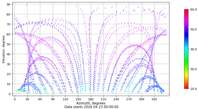
Azimuth-elevation plot for station RIO1. Signal to Noise S1C Data file RIO100ESP_R_2026113.xtr
