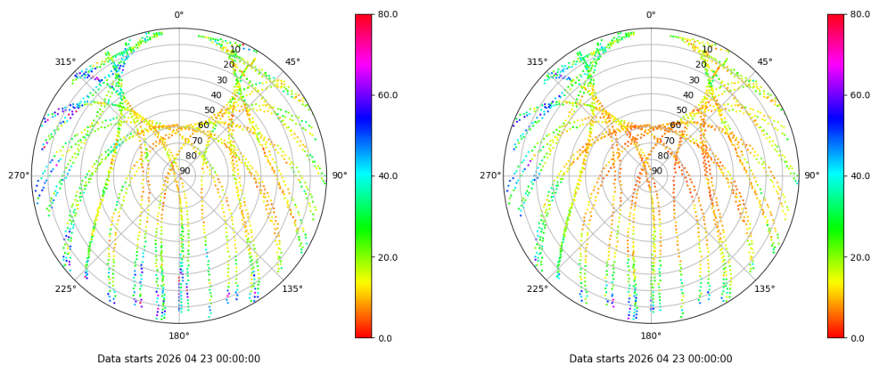
Skyplot for station RIO1. Parameter M1C Data file RIO100ESP_R_2026113.xtr Skyplot for station RIO1. Parameter M2P Data file RIO100ESP_R_2026113.xtr
