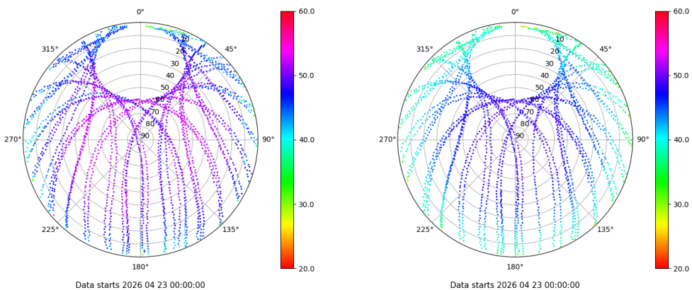
Skyplot for station RIO1. Signal to Noise S1C Data file RIO100ESP_R_2026113.xtr Skyplot for station RIO1. Signal to Noise S2P Data file RIO100ESP_R_2026113.xtr
