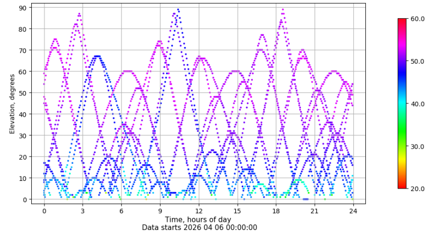
Time-elevation plot for station RIO1. Signal to Noise S1C Data file RIO100ESP_R_2026096.xtr
