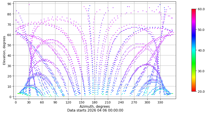
Azimuth-elevation plot for station RIO1. Signal to Noise S1C Data file RIO100ESP_R_2026096.xtr
