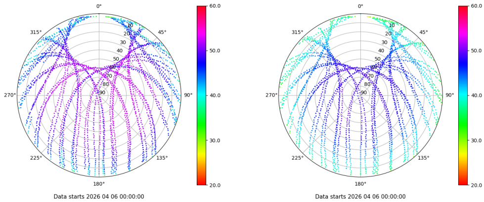
Skyplot for station RIO1. Signal to Noise S1C Data file RIO100ESP_R_2026096.xtr Skyplot for station RIO1. Signal to Noise S2P Data file RIO100ESP_R_2026096.xtr
