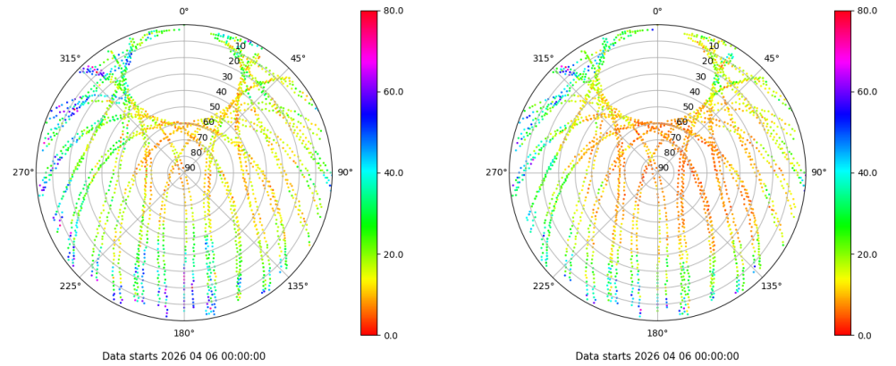
Skyplot for station RIO1. Parameter M1C Data file RIO100ESP_R_2026096.xtr Skyplot for station RIO1. Parameter M2P Data file RIO100ESP_R_2026096.xtr
