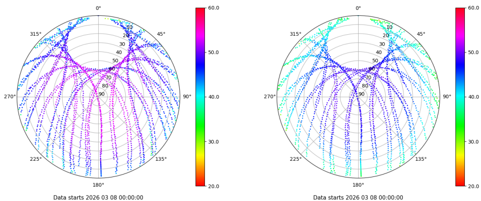
Skyplot for station RIO1. Signal to Noise S1C Data file RIO100ESP_R_2026067.xtr Skyplot for station RIO1. Signal to Noise S2P Data file RIO100ESP_R_2026067.xtr
