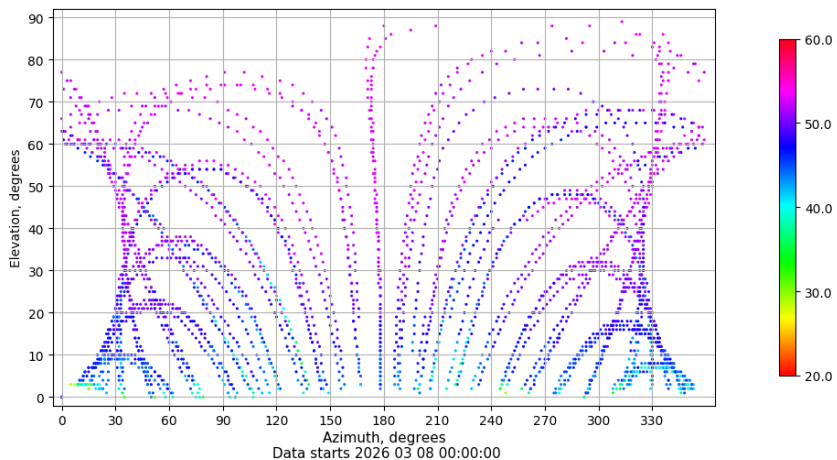
Azimuth-elevation plot for station RIO1. Signal to Noise S1C Data file RIO100ESP_R_2026067.xtr
