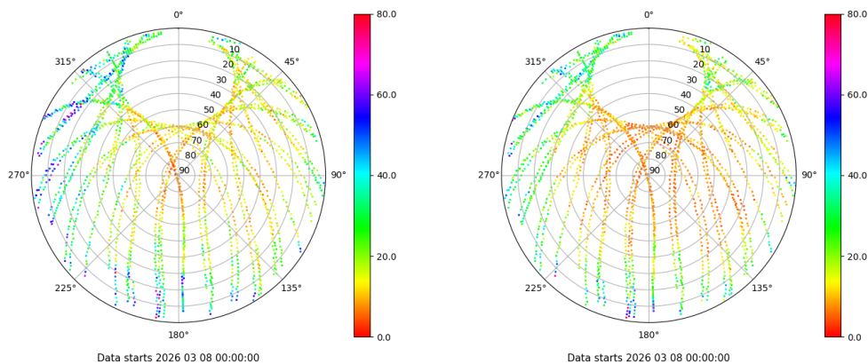
Skyplot for station RIO1. Parameter M1C Data file RIO100ESP_R_2026067.xtr Skyplot for station RIO1. Parameter M2P Data file RIO100ESP_R_2026067.xtr
