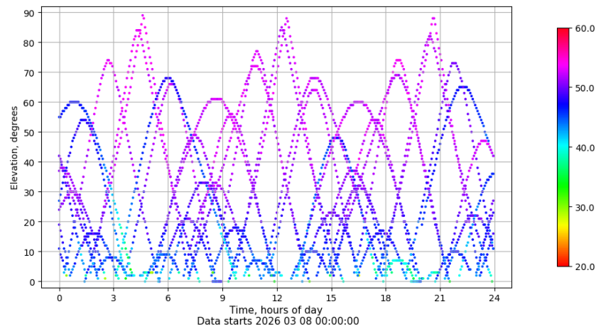
Time-elevation plot for station RIO1. Signal to Noise S1C Data file RIO100ESP_R_2026067.xtr
