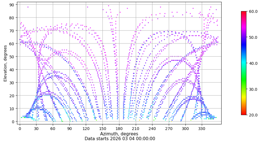
Azimuth-elevation plot for station RIO1. Signal to Noise S1C Data file RIO100ESP_R_2026063.xtr
