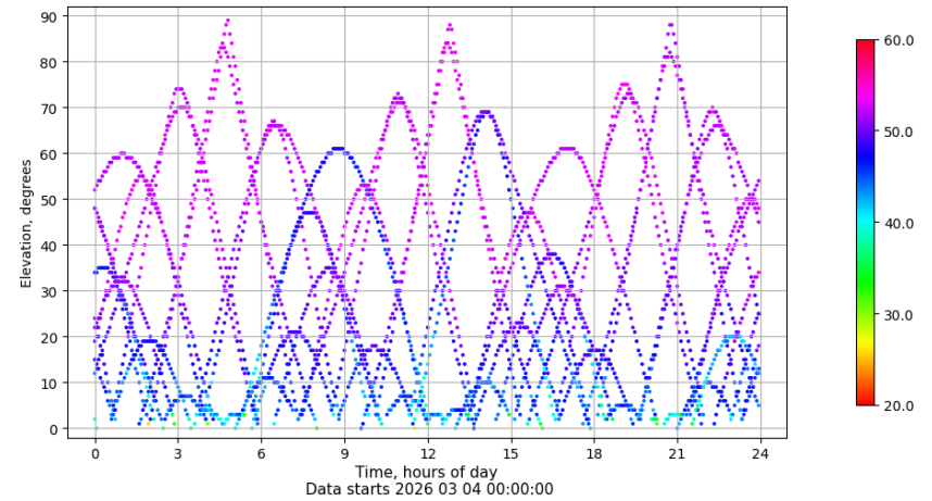
Time-elevation plot for station RIO1. Signal to Noise S1C Data file RIO100ESP_R_2026063.xtr
