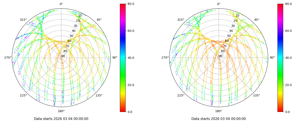
Skyplot for station RIO1. Parameter M1C Data file RIO100ESP_R_2026063.xtr Skyplot for station RIO1. Parameter M2P Data file RIO100ESP_R_2026063.xtr
