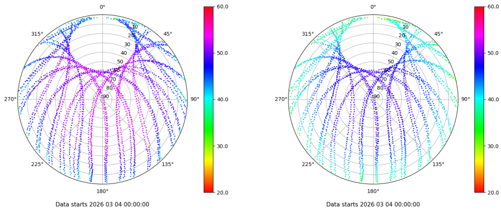
Skyplot for station RIO1. Signal to Noise S1C Data file RIO100ESP_R_2026063.xtr Skyplot for station RIO1. Signal to Noise S2P Data file RIO100ESP_R_2026063.xtr
