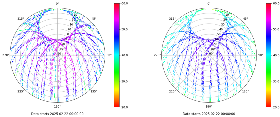
Skyplot for station RIO1. Signal to Noise S1C Data file RIO100ESP_R_2025053.xtr Skyplot for station RIO1. Signal to Noise S2P Data file RIO100ESP_R_2025053.xtr
