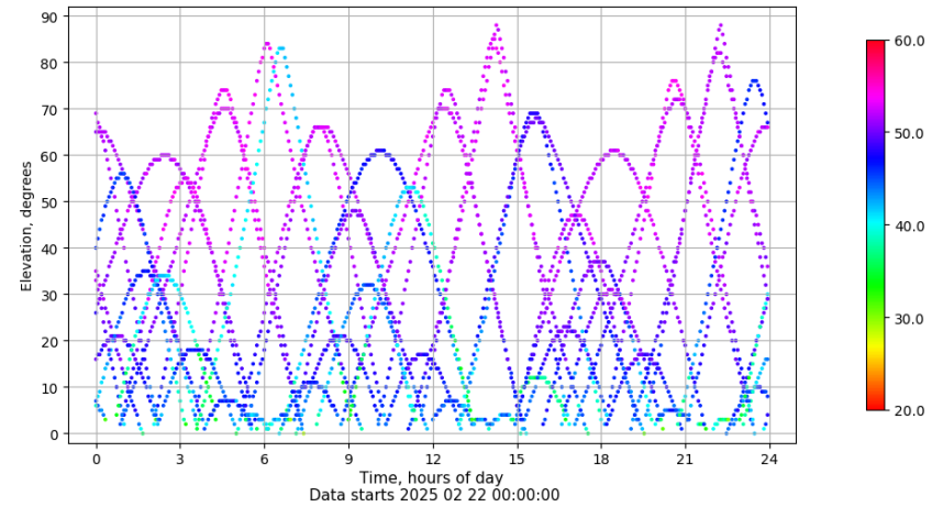
Time-elevation plot for station RIO1. Signal to Noise S1C Data file RIO100ESP_R_2025053.xtr
