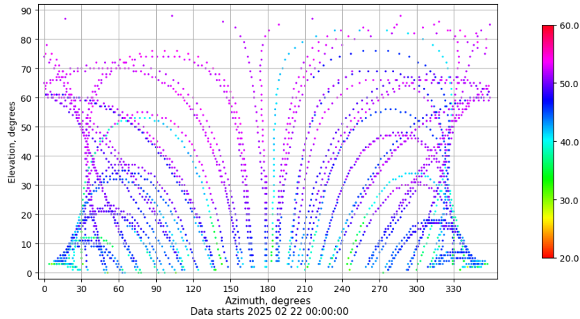
Azimuth-elevation plot for station RIO1. Signal to Noise S1C Data file RIO100ESP_R_2025053.xtr
