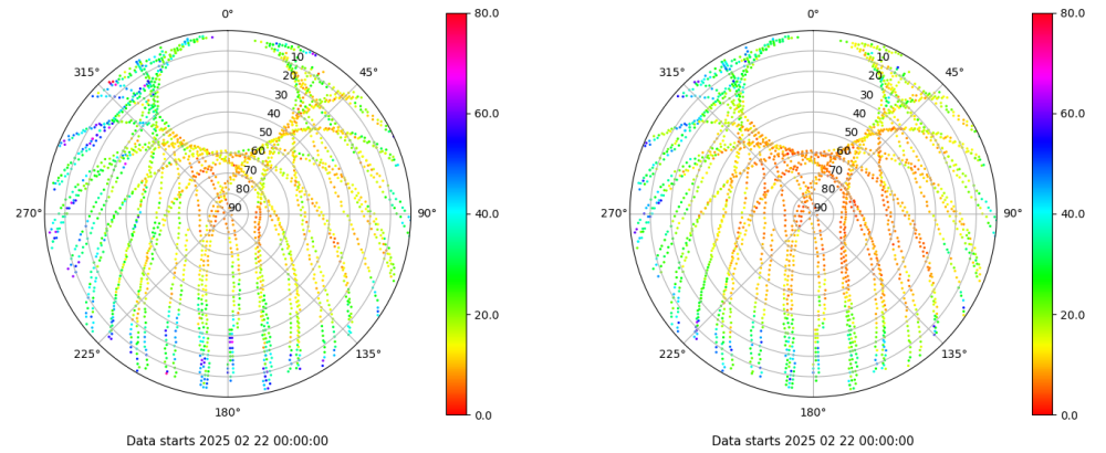
Skyplot for station RIO1. Parameter M1C Data file RIO100ESP_R_2025053.xtr Skyplot for station RIO1. Parameter M2P Data file RIO100ESP_R_2025053.xtr
