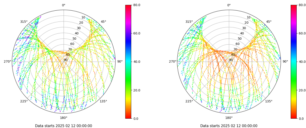
Skyplot for station RIO1. Parameter M1C Data file RIO100ESP_R_2025043.xtr Skyplot for station RIO1. Parameter M2W Data file RIO100ESP_R_2025043.xtr
