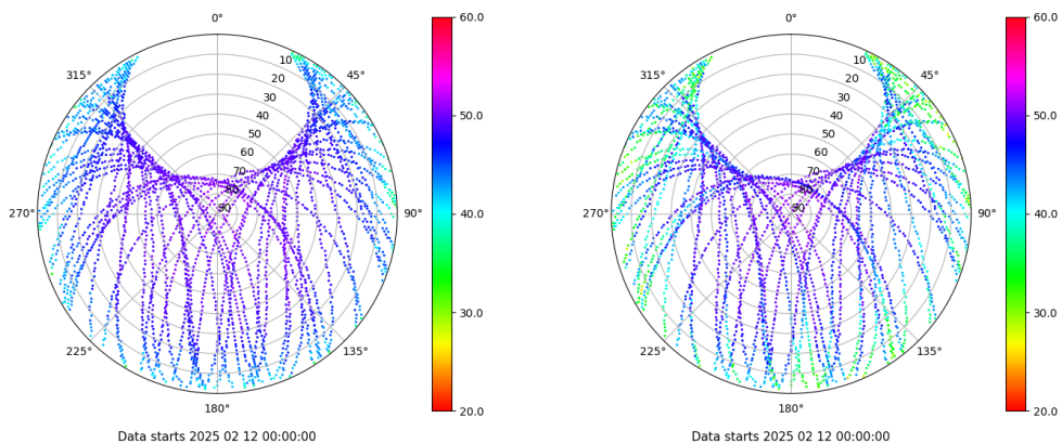
Skyplot for station RIO1. Signal to Noise S1C Data file RIO100ESP_R_2025043.xtr Skyplot for station RIO1. Signal to Noise S2W Data file RIO100ESP_R_2025043.xtr
