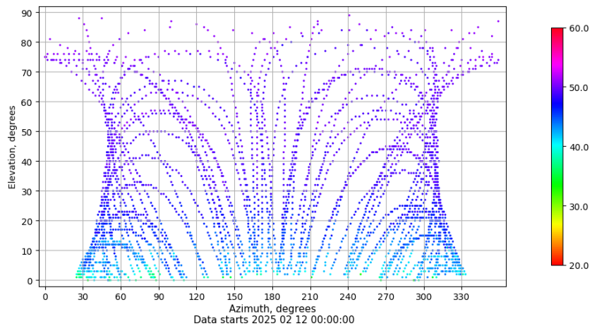
Azimuth-elevation plot for station RIO1. Signal to Noise S1C Data file RIO100ESP_R_2025043.xtr
