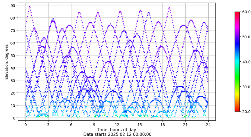
Time-elevation plot for station RIO1. Signal to Noise S1C Data file RIO100ESP_R_2025043.xtr
