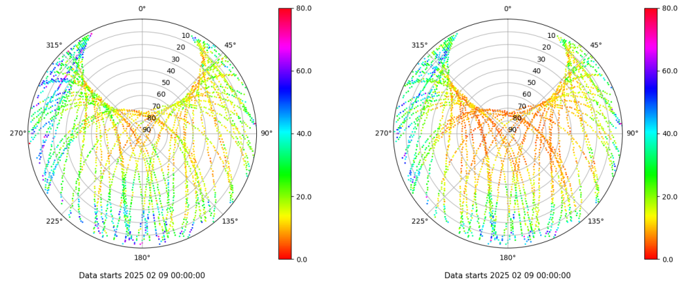
Skyplot for station RIO1. Parameter M1C Data file RIO100ESP_R_2025040.xtr Skyplot for station RIO1. Parameter M2W Data file RIO100ESP_R_2025040.xtr
