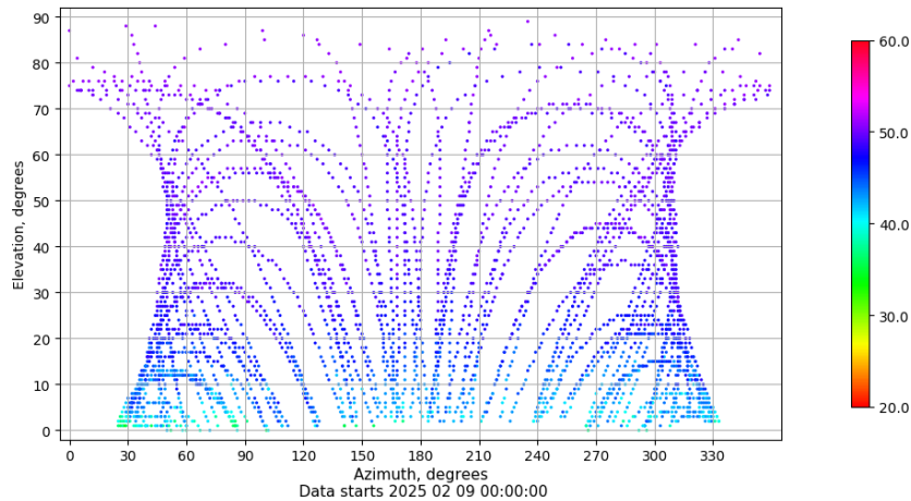
Azimuth-elevation plot for station RIO1. Signal to Noise S1C Data file RIO100ESP_R_2025040.xtr
