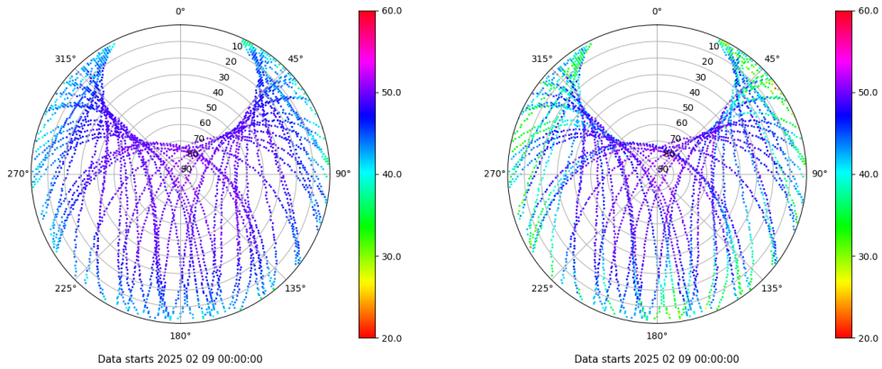
Skyplot for station RIO1. Signal to Noise S1C Data file RIO100ESP_R_2025040.xtr Skyplot for station RIO1. Signal to Noise S2W Data file RIO100ESP_R_2025040.xtr
