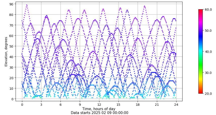
Time-elevation plot for station RIO1. Signal to Noise S1C Data file RIO100ESP_R_2025040.xtr
