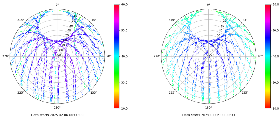
Skyplot for station RIO1. Signal to Noise S1C Data file RIO100ESP_R_2025037.xtr Skyplot for station RIO1. Signal to Noise S2P Data file RIO100ESP_R_2025037.xtr
