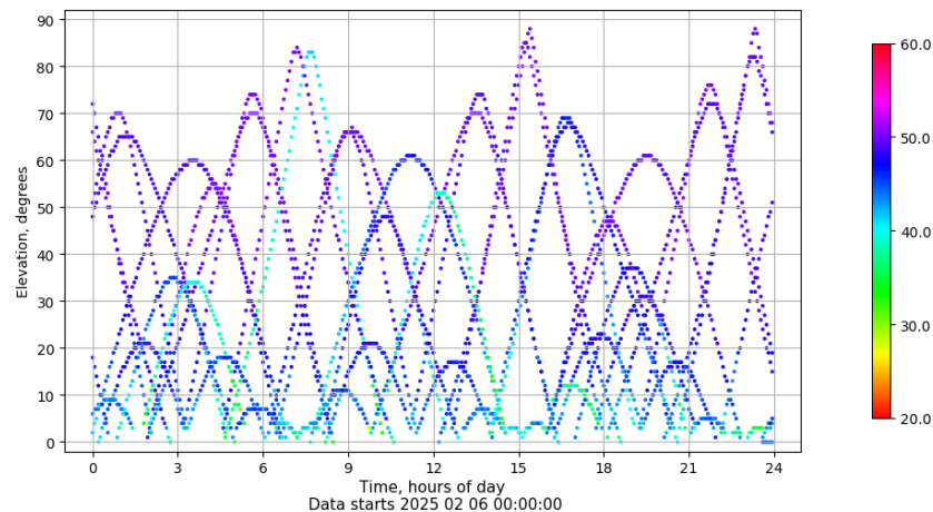
Time-elevation plot for station RIO1. Signal to Noise S1C Data file RIO100ESP_R_2025037.xtr
