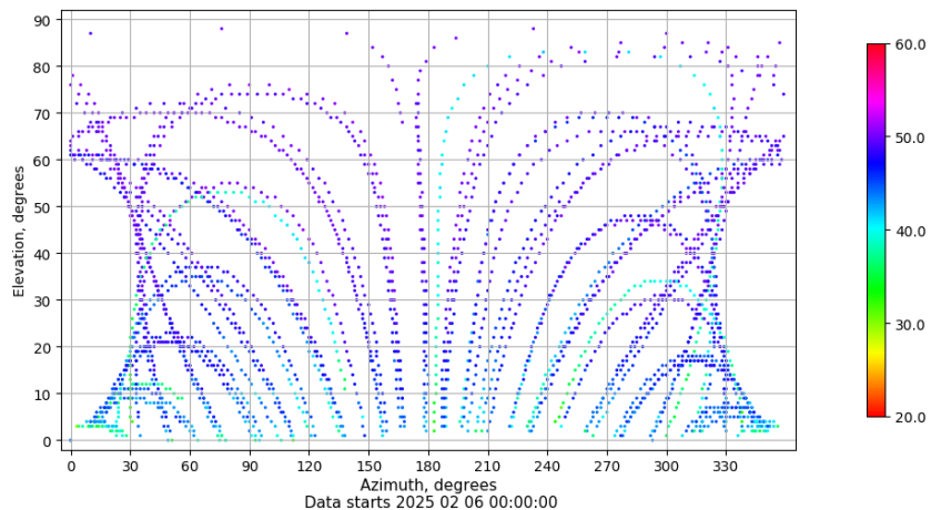
Azimuth-elevation plot for station RIO1. Signal to Noise S1C Data file RIO100ESP_R_2025037.xtr
