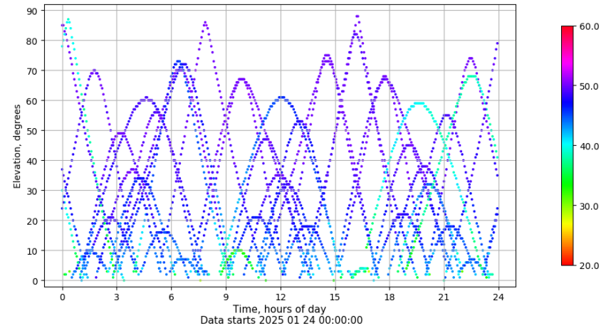
Time-elevation plot for station RIO1. Signal to Noise S1C Data file RIO100ESP_R_2025024.xtr
