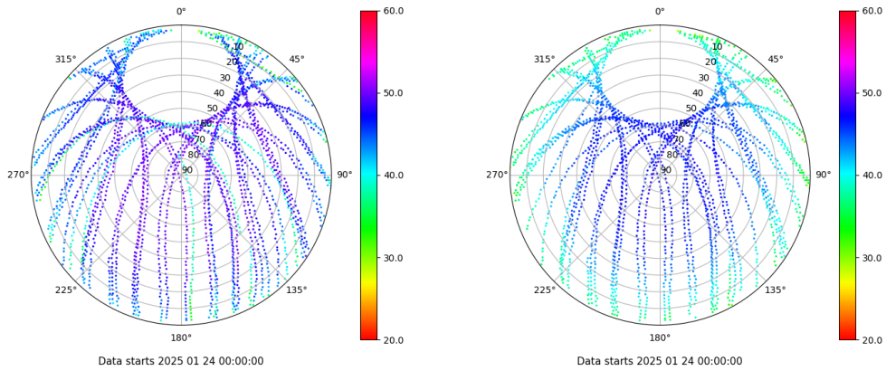
Skyplot for station RIO1. Signal to Noise S1C Data file RIO100ESP_R_2025024.xtr Skyplot for station RIO1. Signal to Noise S2P Data file RIO100ESP_R_2025024.xtr
