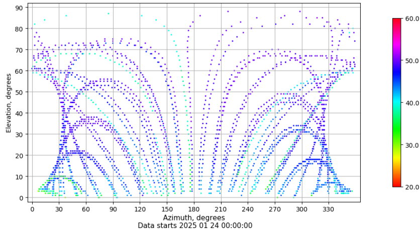
Azimuth-elevation plot for station RIO1. Signal to Noise S1C Data file RIO100ESP_R_2025024.xtr
