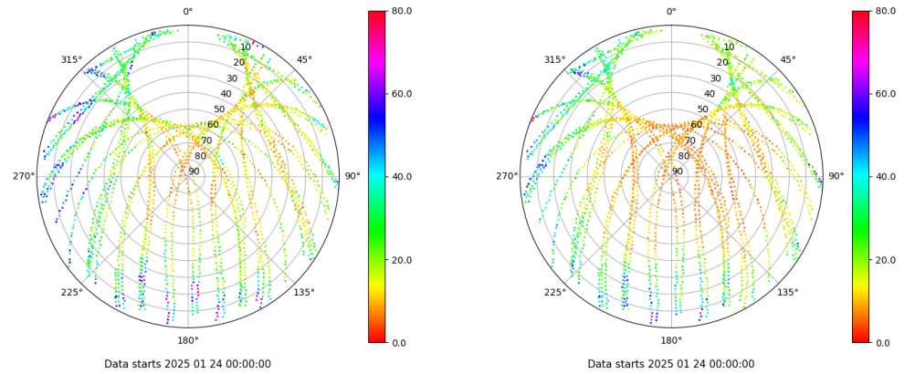
Skyplot for station RIO1. Parameter M1C Data file RIO100ESP_R_2025024.xtr Skyplot for station RIO1. Parameter M2P Data file RIO100ESP_R_2025024.xtr
