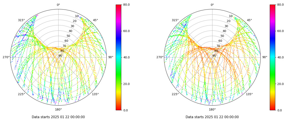
Skyplot for station RIO1. Parameter M1C Data file RIO100ESP_R_2025022.xtr Skyplot for station RIO1. Parameter M2W Data file RIO100ESP_R_2025022.xtr
