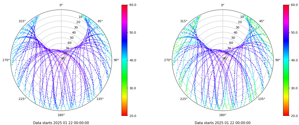
Skyplot for station RIO1. Signal to Noise S1C Data file RIO100ESP_R_2025022.xtr Skyplot for station RIO1. Signal to Noise S2W Data file RIO100ESP_R_2025022.xtr
