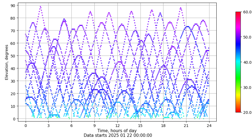
Time-elevation plot for station RIO1. Signal to Noise S1C Data file RIO100ESP_R_2025022.xtr
