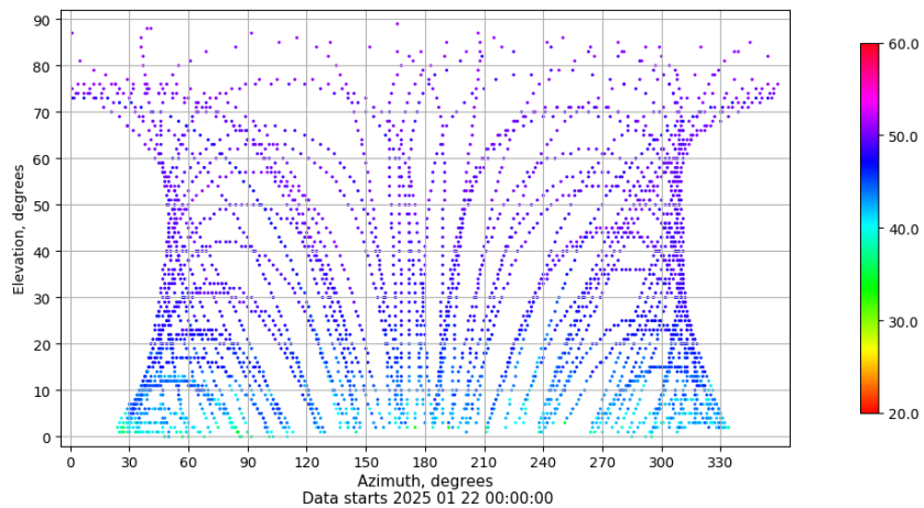
Azimuth-elevation plot for station RIO1. Signal to Noise S1C Data file RIO100ESP_R_2025022.xtr
