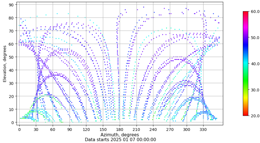
Azimuth-elevation plot for station RIO1. Signal to Noise S1C Data file RIO100ESP_R_2025007.xtr
