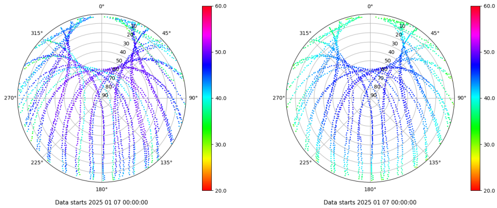
Skyplot for station RIO1. Signal to Noise S1C Data file RIO100ESP_R_2025007.xtr Skyplot for station RIO1. Signal to Noise S2P Data file RIO100ESP_R_2025007.xtr
