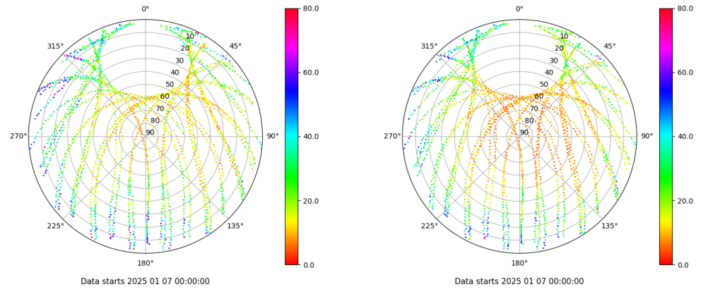
Skyplot for station RIO1. Parameter M1C Data file RIO100ESP_R_2025007.xtr Skyplot for station RIO1. Parameter M2P Data file RIO100ESP_R_2025007.xtr
