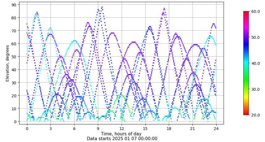
Time-elevation plot for station RIO1. Signal to Noise S1C Data file RIO100ESP_R_2025007.xtr
