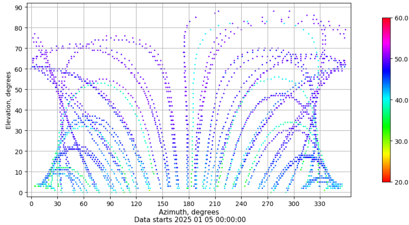
Azimuth-elevation plot for station RIO1. Signal to Noise S1C Data file RIO100ESP_R_2025005.xtr
