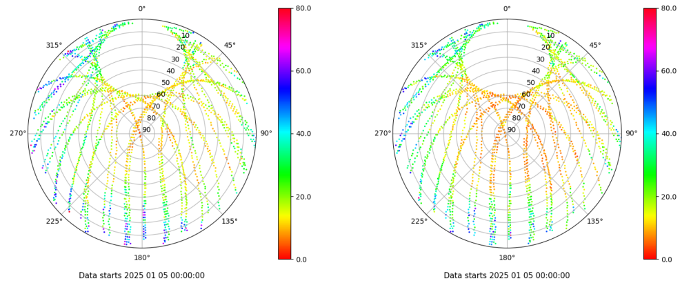
Skyplot for station RIO1. Parameter M1C Data file RIO100ESP_R_2025005.xtr Skyplot for station RIO1. Parameter M2P Data file RIO100ESP_R_2025005.xtr
