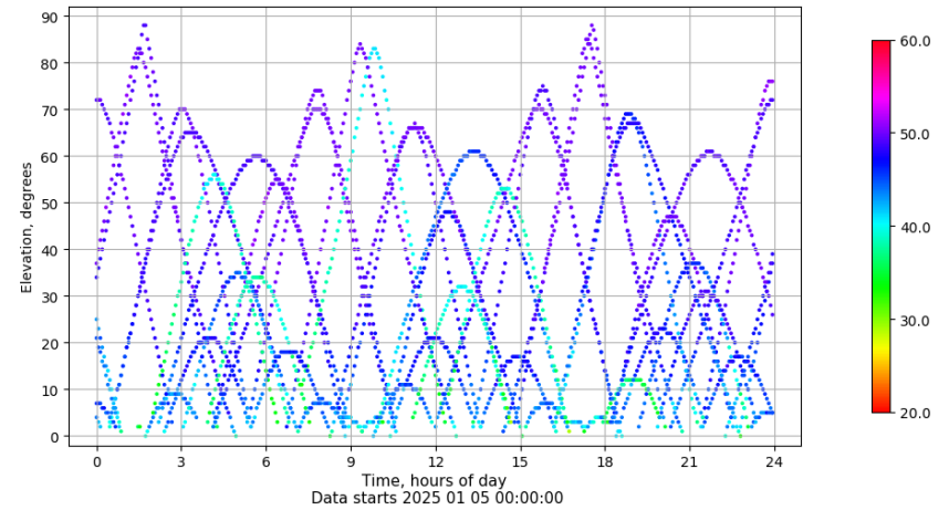
Time-elevation plot for station RIO1. Signal to Noise S1C Data file RIO100ESP_R_2025005.xtr
