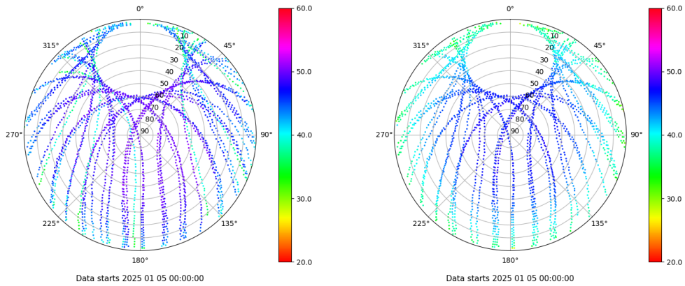
Skyplot for station RIO1. Signal to Noise S1C Data file RIO100ESP_R_2025005.xtr Skyplot for station RIO1. Signal to Noise S2P Data file RIO100ESP_R_2025005.xtr
