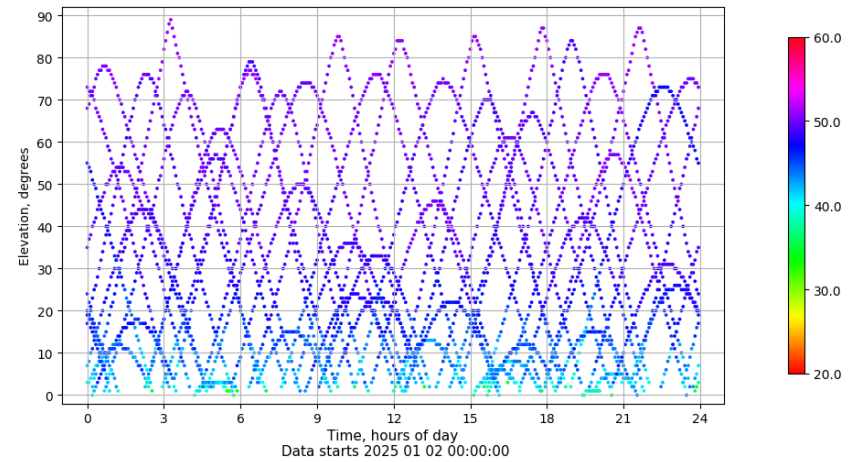
Time-elevation plot for station RIO1. Signal to Noise S1C Data file RIO100ESP_R_2025002.xtr
