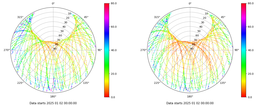
Skyplot for station RIO1. Parameter M1C Data file RIO100ESP_R_2025002.xtr Skyplot for station RIO1. Parameter M2W Data file RIO100ESP_R_2025002.xtr
