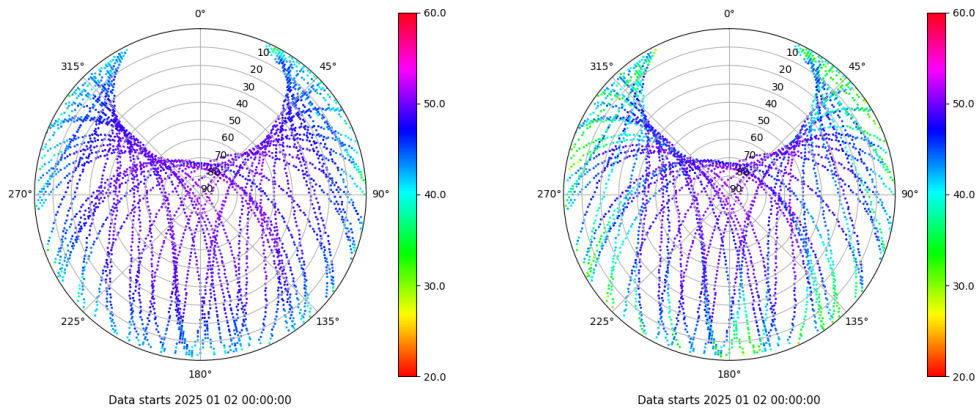
Skyplot for station RIO1. Signal to Noise S1C Data file RIO100ESP_R_2025002.xtr Skyplot for station RIO1. Signal to Noise S2W Data file RIO100ESP_R_2025002.xtr
