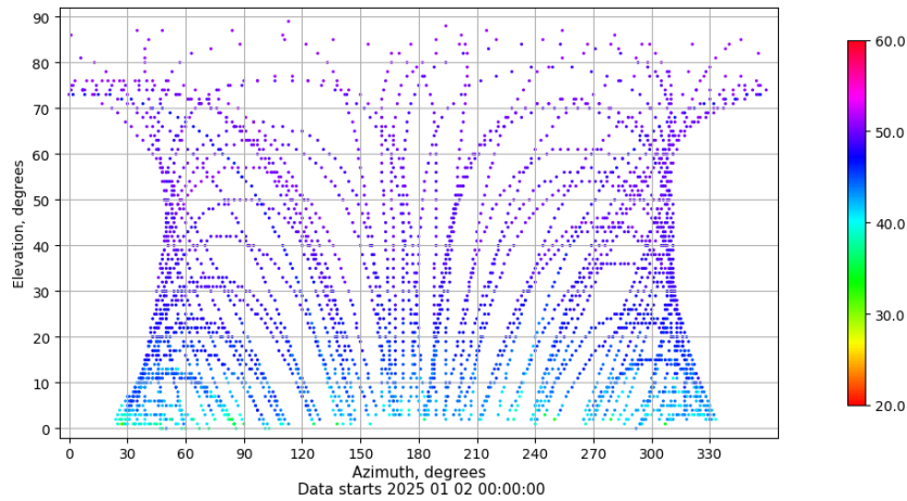
Azimuth-elevation plot for station RIO1. Signal to Noise S1C Data file RIO100ESP_R_2025002.xtr
