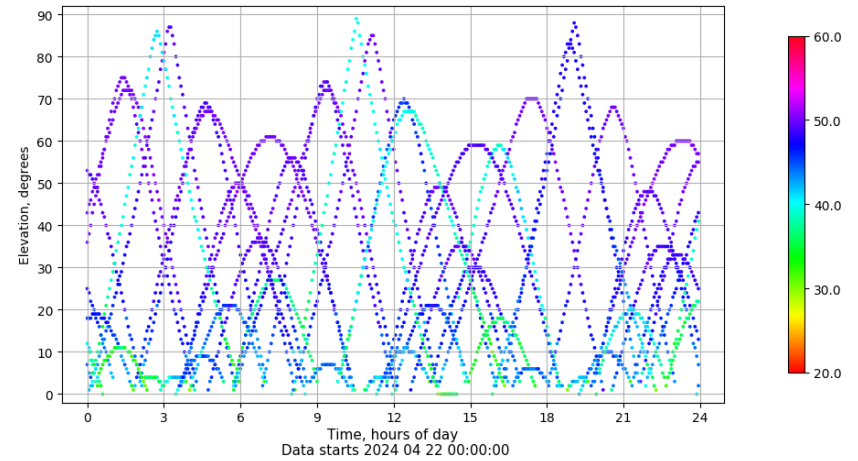
Time-elevation plot for station RIO1. Signal to Noise S1C Data file RIO100ESP_R_2024113.xtr
