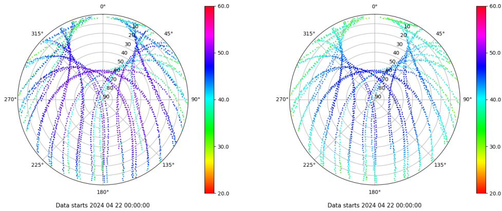
Skyplot for station RIO1. Signal to Noise S1C Data file RIO100ESP_R_2024113.xtr Skyplot for station RIO1. Signal to Noise S2P Data file RIO100ESP_R_2024113.xtr
