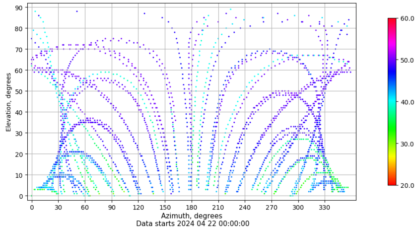
Azimuth-elevation plot for station RIO1. Signal to Noise S1C Data file RIO100ESP_R_2024113.xtr
