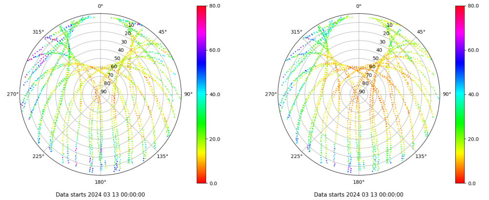
Skyplot for station RIO1. Parameter M1C Data file RIO100ESP_R_2024073.xtr Skyplot for station RIO1. Parameter M2P Data file RIO100ESP_R_2024073.xtr
