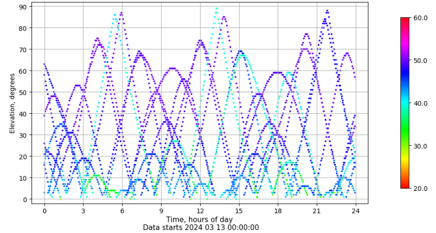
Time-elevation plot for station RIO1. Signal to Noise S1C Data file RIO100ESP_R_2024073.xtr
