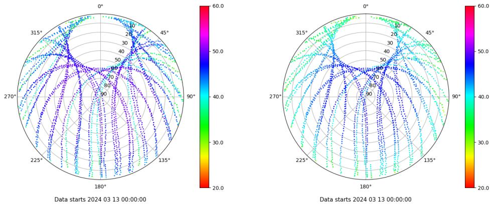
Skyplot for station RIO1. Signal to Noise S1C Data file RIO100ESP_R_2024073.xtr Skyplot for station RIO1. Signal to Noise S2P Data file RIO100ESP_R_2024073.xtr
