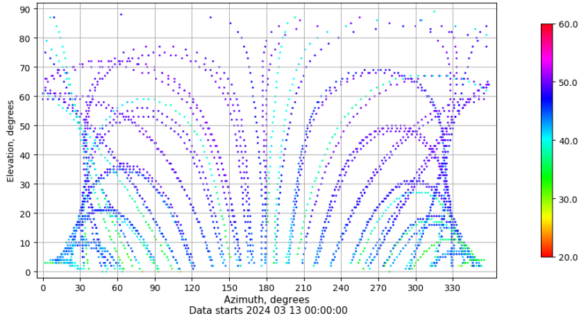
Azimuth-elevation plot for station RIO1. Signal to Noise S1C Data file RIO100ESP_R_2024073.xtr
