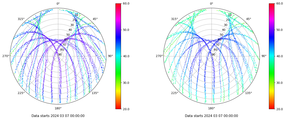
Skyplot for station RIO1. Signal to Noise S1C Data file RIO100ESP_R_2024067.xtr Skyplot for station RIO1. Signal to Noise S2P Data file RIO100ESP_R_2024067.xtr
