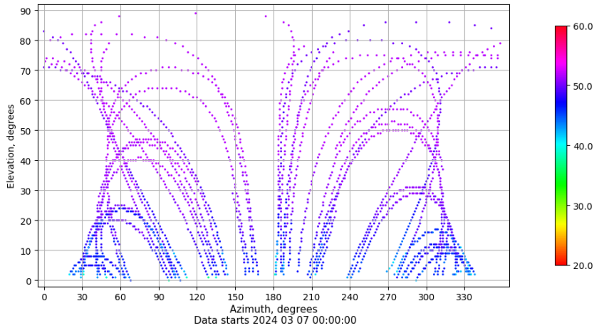
Azimuth-elevation plot for station RIO1. Signal to Noise S1C Data file RIO100ESP_R_2024067.xtr
