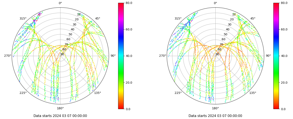
Skyplot for station RIO1. Parameter M1C Data file RIO100ESP_R_2024067.xtr Skyplot for station RIO1. Parameter M5Q Data file RIO100ESP_R_2024067.xtr
