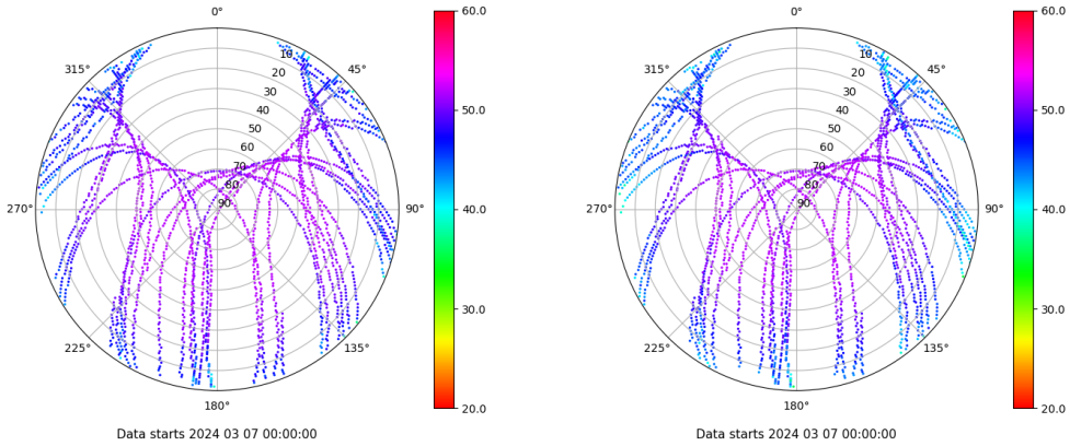
Skyplot for station RIO1. Signal to Noise S1C Data file RIO100ESP_R_2024067.xtr Skyplot for station RIO1. Signal to Noise S5Q Data file RIO100ESP_R_2024067.xtr
