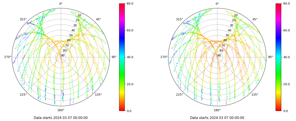
Skyplot for station RIO1. Parameter M1C Data file RIO100ESP_R_2024067.xtr Skyplot for station RIO1. Parameter M2P Data file RIO100ESP_R_2024067.xtr
