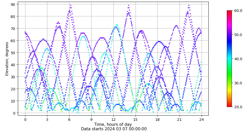
Time-elevation plot for station RIO1. Signal to Noise S1C Data file RIO100ESP_R_2024067.xtr
