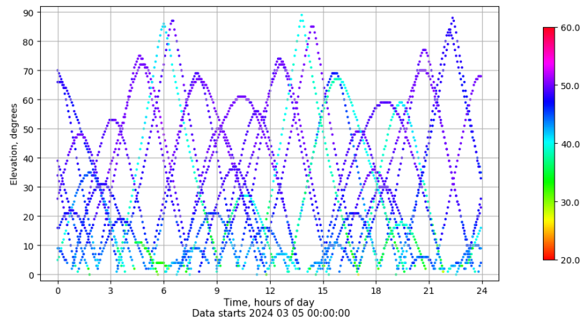
Time-elevation plot for station RIO1. Signal to Noise S1C Data file RIO100ESP_R_2024065.xtr
