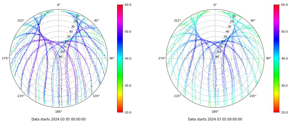
Skyplot for station RIO1. Signal to Noise S1C Data file RIO100ESP_R_2024065.xtr Skyplot for station RIO1. Signal to Noise S2P Data file RIO100ESP_R_2024065.xtr
