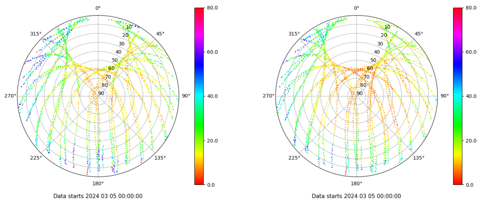
Skyplot for station RIO1. Parameter M1C Data file RIO100ESP_R_2024065.xtr Skyplot for station RIO1. Parameter M2P Data file RIO100ESP_R_2024065.xtr
