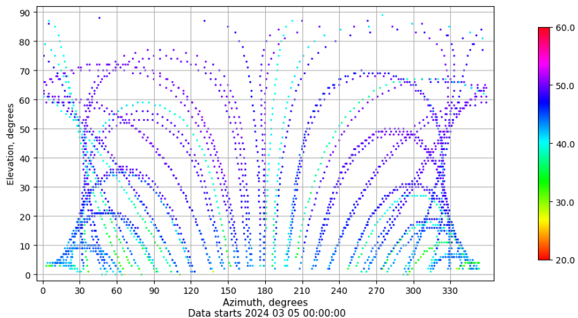
Azimuth-elevation plot for station RIO1. Signal to Noise S1C Data file RIO100ESP_R_2024065.xtr
