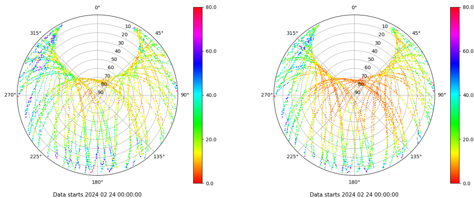
Skyplot for station RIO1. Parameter M1C Data file RIO100ESP_R_2024055.xtr Skyplot for station RIO1. Parameter M2W Data file RIO100ESP_R_2024055.xtr
