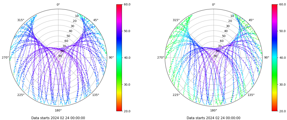
Skyplot for station RIO1. Signal to Noise S1C Data file RIO100ESP_R_2024055.xtr Skyplot for station RIO1. Signal to Noise S2W Data file RIO100ESP_R_2024055.xtr
