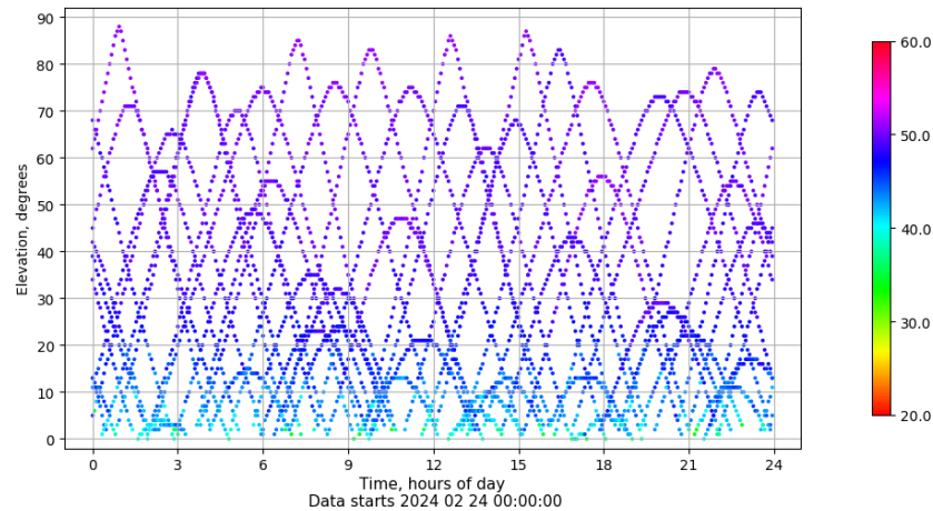
Time-elevation plot for station RIO1. Signal to Noise S1C Data file RIO100ESP_R_2024055.xtr
