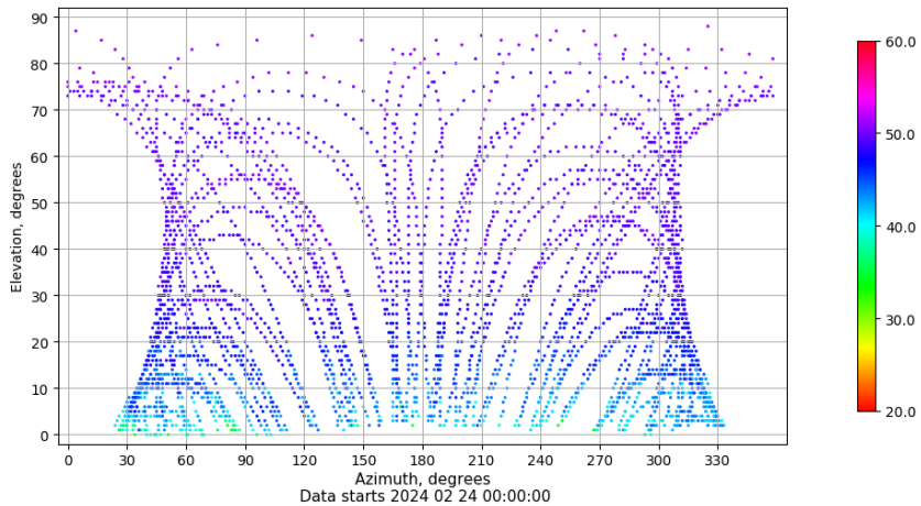
Azimuth-elevation plot for station RIO1. Signal to Noise S1C Data file RIO100ESP_R_2024055.xtr
