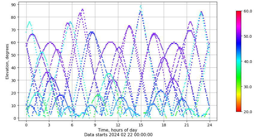
Time-elevation plot for station RIO1. Signal to Noise S1C Data file RIO100ESP_R_2024053.xtr
