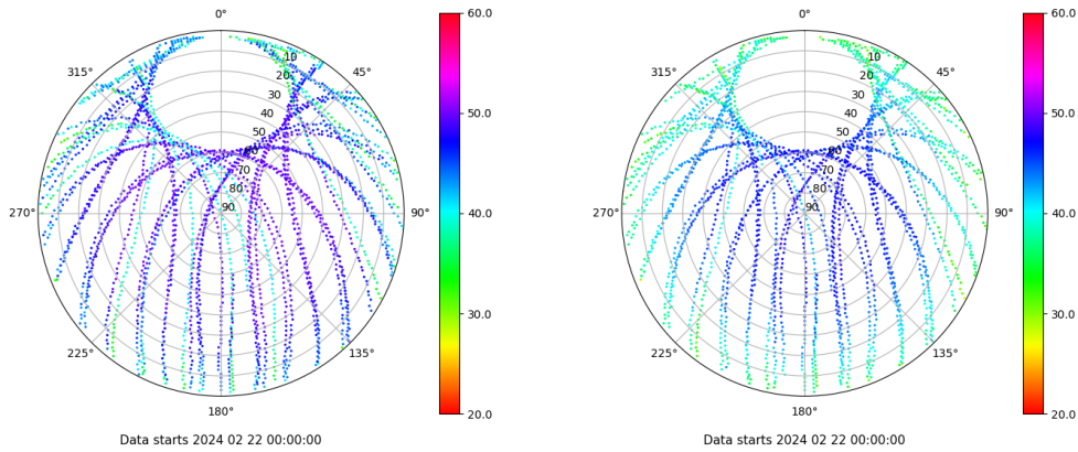
Skyplot for station RIO1. Signal to Noise S1C Data file RIO100ESP_R_2024053.xtr Skyplot for station RIO1. Signal to Noise S2P Data file RIO100ESP_R_2024053.xtr
