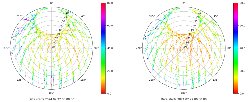
Skyplot for station RIO1. Parameter M1C Data file RIO100ESP_R_2024053.xtr Skyplot for station RIO1. Parameter M2P Data file RIO100ESP_R_2024053.xtr
