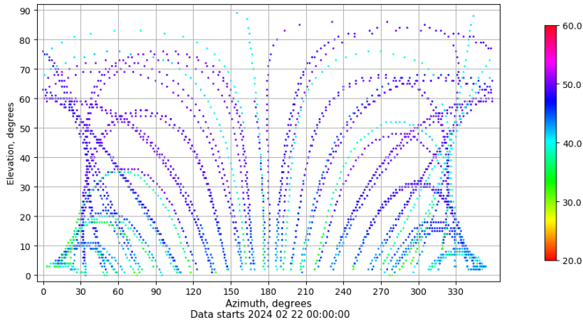
Azimuth-elevation plot for station RIO1. Signal to Noise S1C Data file RIO100ESP_R_2024053.xtr
