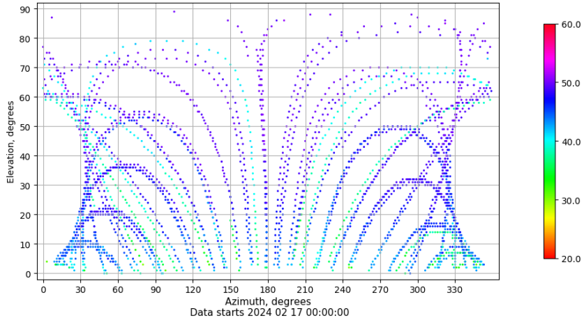
Azimuth-elevation plot for station RIO1. Signal to Noise S1C Data file RIO100ESP_R_2024048.xtr
