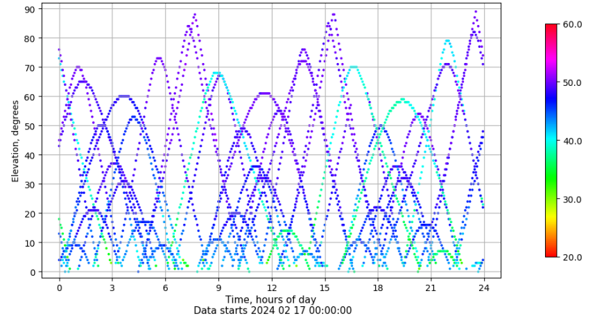
Time-elevation plot for station RIO1. Signal to Noise S1C Data file RIO100ESP_R_2024048.xtr
