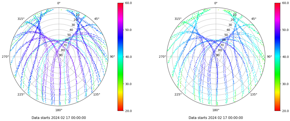
Skyplot for station RIO1. Signal to Noise S1C Data file RIO100ESP_R_2024048.xtr Skyplot for station RIO1. Signal to Noise S2P Data file RIO100ESP_R_2024048.xtr
