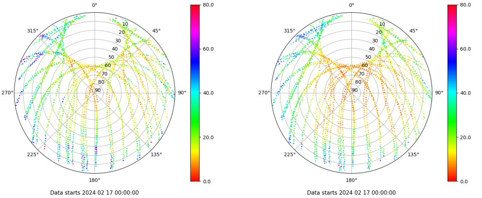
Skyplot for station RIO1. Parameter M1C Data file RIO100ESP_R_2024048.xtr Skyplot for station RIO1. Parameter M2P Data file RIO100ESP_R_2024048.xtr
