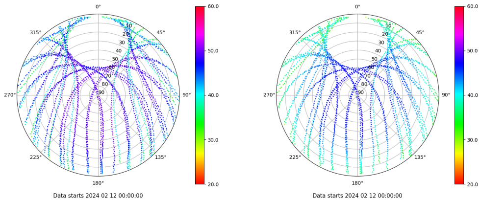
Skyplot for station RIO1. Signal to Noise S1C Data file RIO100ESP_R_2024043.xtr Skyplot for station RIO1. Signal to Noise S2P Data file RIO100ESP_R_2024043.xtr
