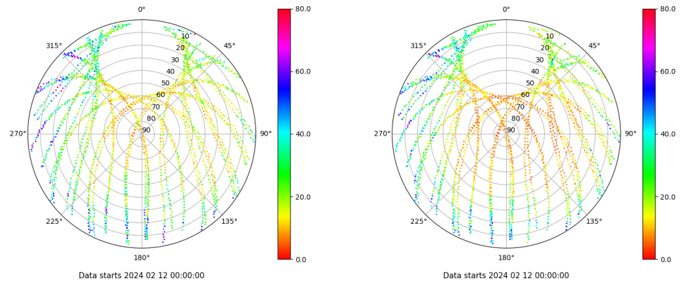
Skyplot for station RIO1. Parameter M1C Data file RIO100ESP_R_2024043.xtr Skyplot for station RIO1. Parameter M2P Data file RIO100ESP_R_2024043.xtr
