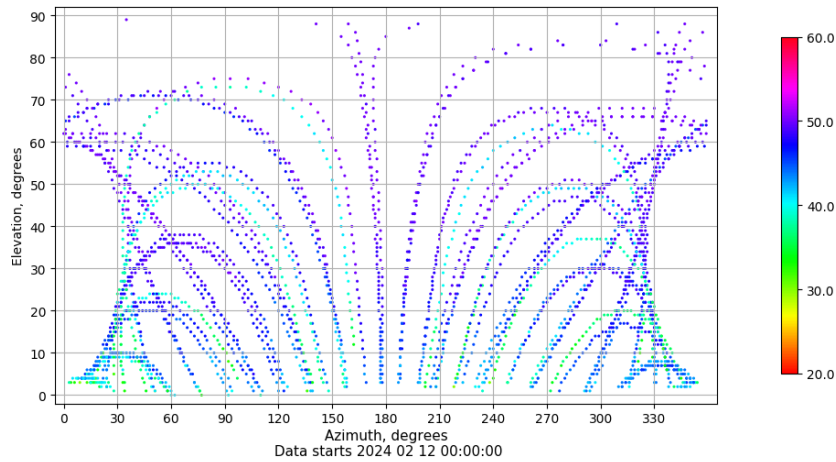
Azimuth-elevation plot for station RIO1. Signal to Noise S1C Data file RIO100ESP_R_2024043.xtr
