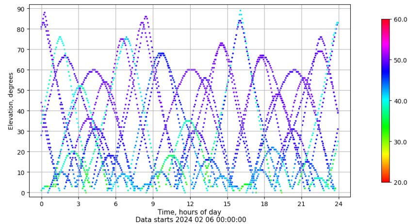
Time-elevation plot for station RIO1. Signal to Noise S1C Data file RIO100ESP_R_2024037.xtr
