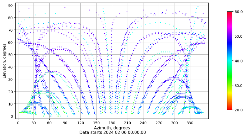
Azimuth-elevation plot for station RIO1. Signal to Noise S1C Data file RIO100ESP_R_2024037.xtr
