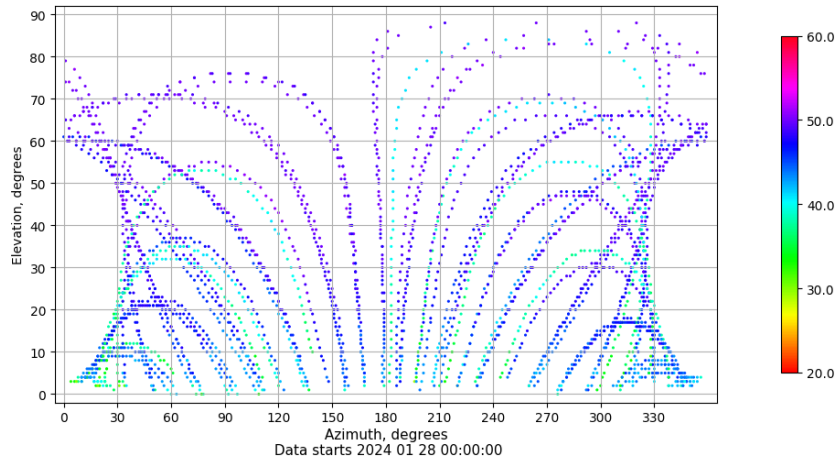
Azimuth-elevation plot for station RIO1. Signal to Noise S1C Data file RIO100ESP_R_2024028.xtr
