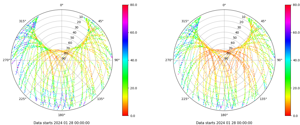
Skyplot for station RIO1. Parameter M1C Data file RIO100ESP_R_2024028.xtr Skyplot for station RIO1. Parameter M2W Data file RIO100ESP_R_2024028.xtr
