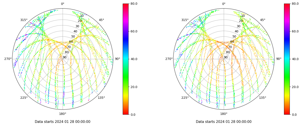
Skyplot for station RIO1. Parameter M1C Data file RIO100ESP_R_2024028.xtr Skyplot for station RIO1. Parameter M2P Data file RIO100ESP_R_2024028.xtr
