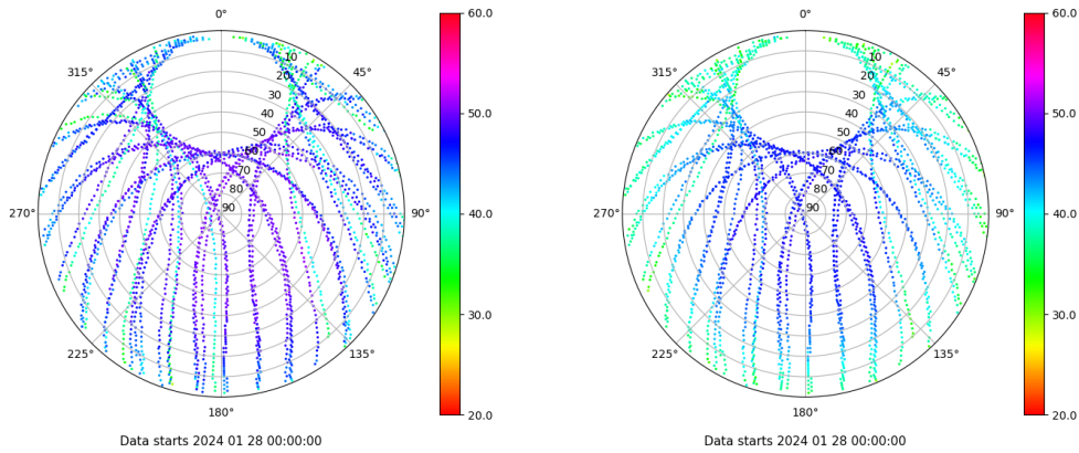
Skyplot for station RIO1. Signal to Noise S1C Data file RIO100ESP_R_2024028.xtr Skyplot for station RIO1. Signal to Noise S2P Data file RIO100ESP_R_2024028.xtr
