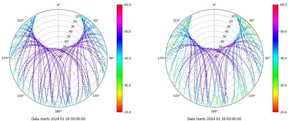
Skyplot for station RIO1. Signal to Noise S1C Data file RIO100ESP_R_2024028.xtr Skyplot for station RIO1. Signal to Noise S2W Data file RIO100ESP_R_2024028.xtr
