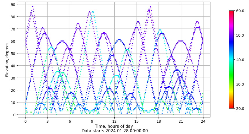
Time-elevation plot for station RIO1. Signal to Noise S1C Data file RIO100ESP_R_2024028.xtr
