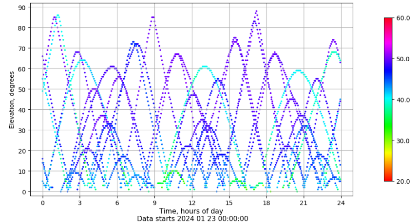
Time-elevation plot for station RIO1. Signal to Noise S1C Data file RIO100ESP_R_2024023.xtr
