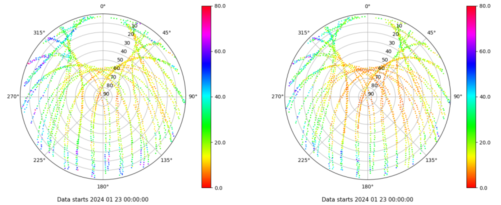
Skyplot for station RIO1. Parameter M1C Data file RIO100ESP_R_2024023.xtr Skyplot for station RIO1. Parameter M2P Data file RIO100ESP_R_2024023.xtr
