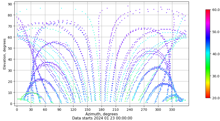
Azimuth-elevation plot for station RIO1. Signal to Noise S1C Data file RIO100ESP_R_2024023.xtr
