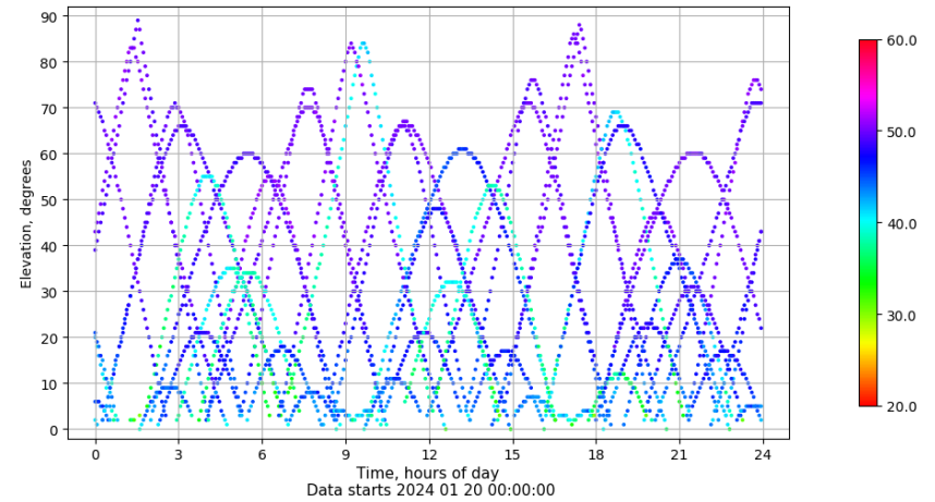
Time-elevation plot for station RIO1. Signal to Noise S1C Data file RIO100ESP_R_2024020.xtr
