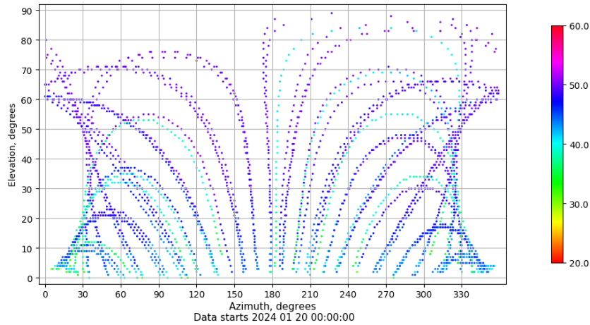
Azimuth-elevation plot for station RIO1. Signal to Noise S1C Data file RIO100ESP_R_2024020.xtr
