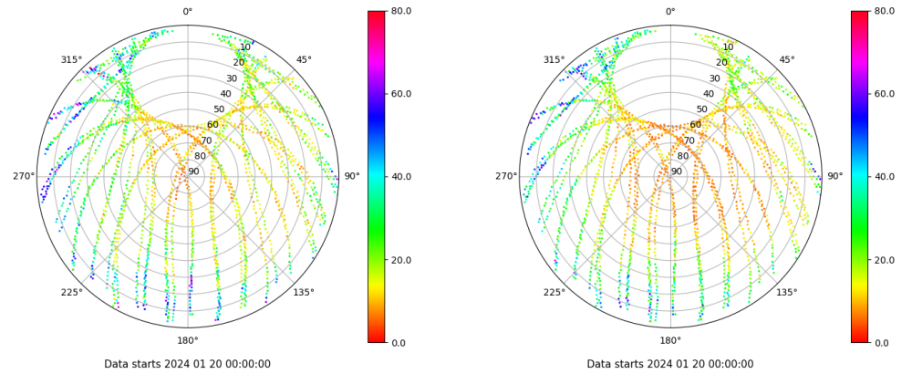
Skyplot for station RIO1. Parameter M1C Data file RIO100ESP_R_2024020.xtr Skyplot for station RIO1. Parameter M2P Data file RIO100ESP_R_2024020.xtr
