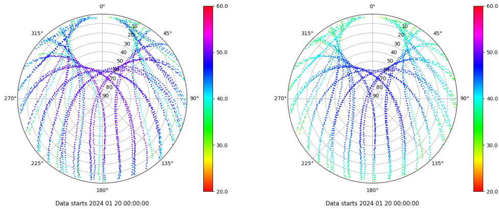
Skyplot for station RIO1. Signal to Noise S1C Data file RIO100ESP_R_2024020.xtr Skyplot for station RIO1. Signal to Noise S2P Data file RIO100ESP_R_2024020.xtr
