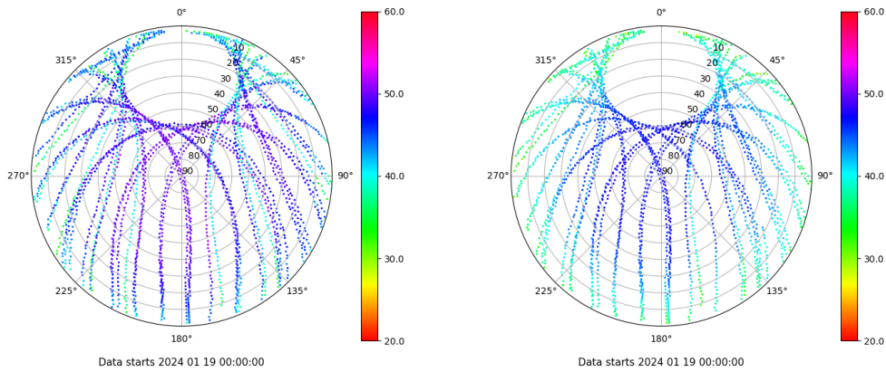
Skyplot for station RIO1. Signal to Noise S1C Data file RIO100ESP_R_2024019.xtr Skyplot for station RIO1. Signal to Noise S2P Data file RIO100ESP_R_2024019.xtr
