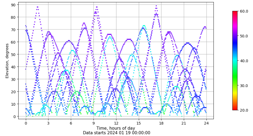
Time-elevation plot for station RIO1. Signal to Noise S1C Data file RIO100ESP_R_2024019.xtr
