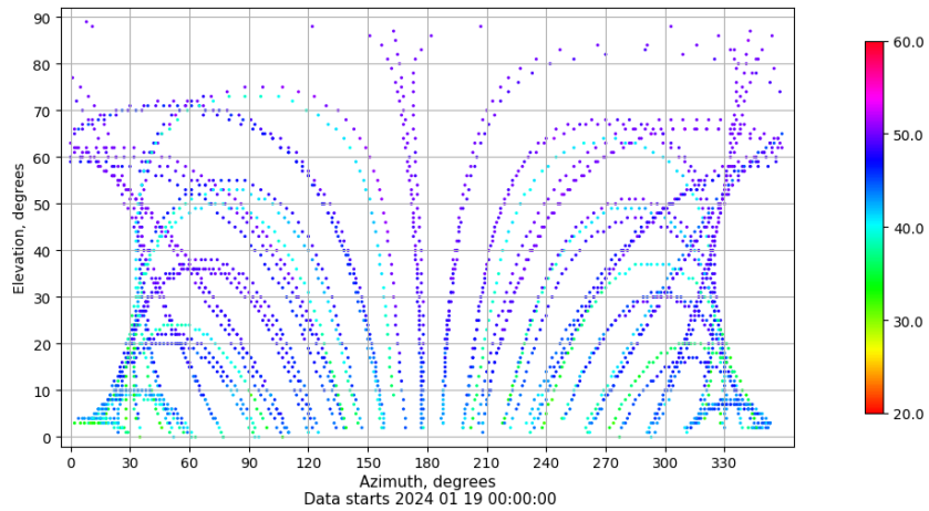
Azimuth-elevation plot for station RIO1. Signal to Noise S1C Data file RIO100ESP_R_2024019.xtr
