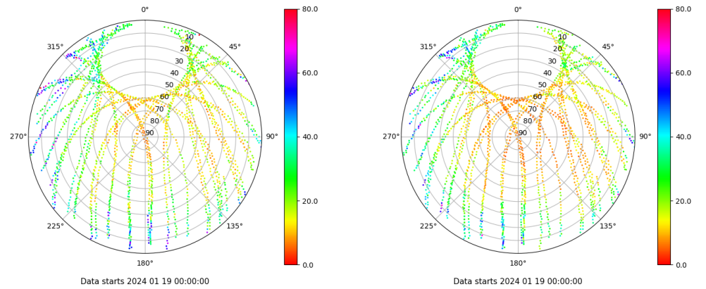
Skyplot for station RIO1. Parameter M1C Data file RIO100ESP_R_2024019.xtr Skyplot for station RIO1. Parameter M2P Data file RIO100ESP_R_2024019.xtr
