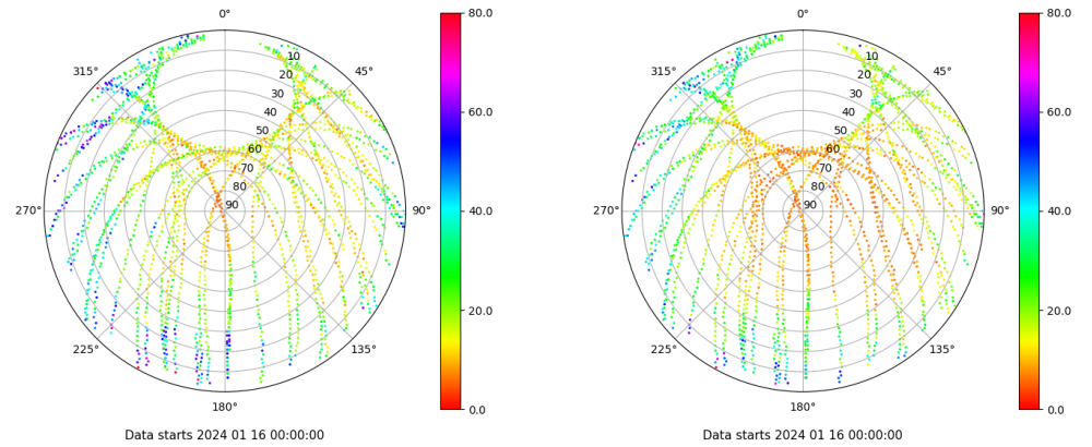
Skyplot for station RIO1. Parameter M1C Data file RIO100ESP_R_2024016.xtr Skyplot for station RIO1. Parameter M2P Data file RIO100ESP_R_2024016.xtr
