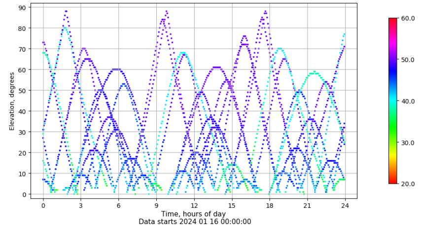
Time-elevation plot for station RIO1. Signal to Noise S1C Data file RIO100ESP_R_2024016.xtr
