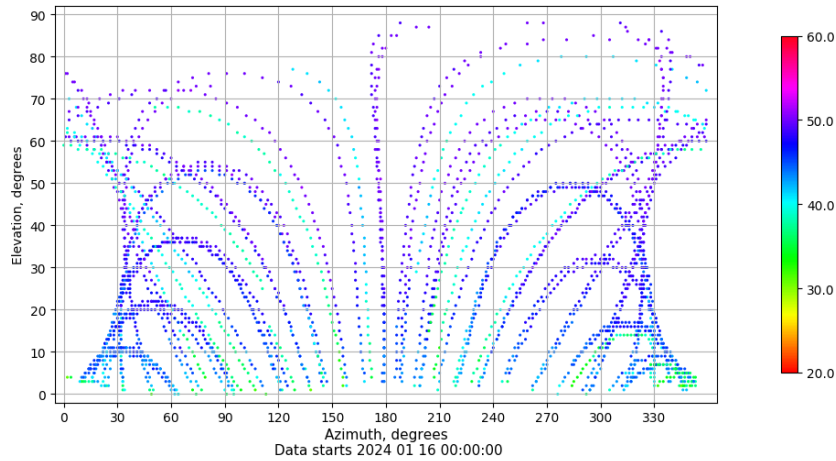
Azimuth-elevation plot for station RIO1. Signal to Noise S1C Data file RIO100ESP_R_2024016.xtr
