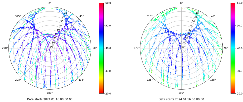
Skyplot for station RIO1. Signal to Noise S1C Data file RIO100ESP_R_2024016.xtr Skyplot for station RIO1. Signal to Noise S2P Data file RIO100ESP_R_2024016.xtr
