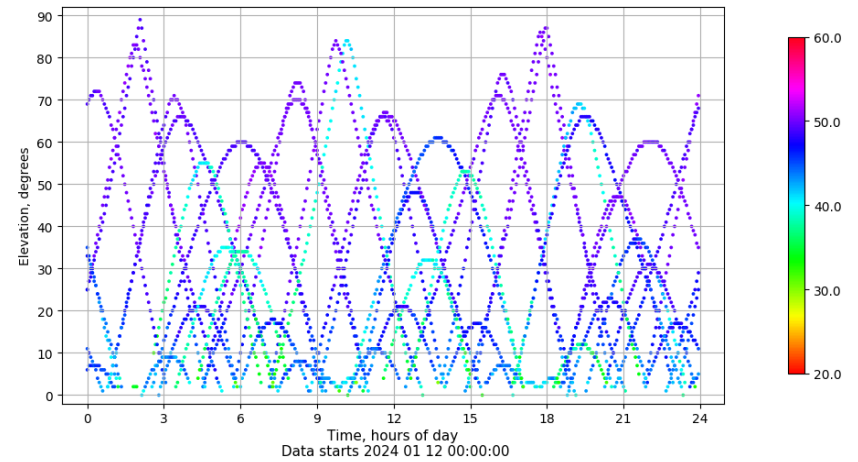
Time-elevation plot for station RIO1. Signal to Noise S1C Data file RIO100ESP_R_2024012.xtr
