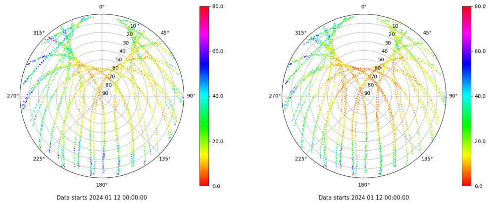
Skyplot for station RIO1. Parameter M1C Data file RIO100ESP_R_2024012.xtr Skyplot for station RIO1. Parameter M2P Data file RIO100ESP_R_2024012.xtr
