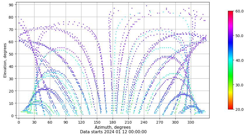
Azimuth-elevation plot for station RIO1. Signal to Noise S1C Data file RIO100ESP_R_2024012.xtr
