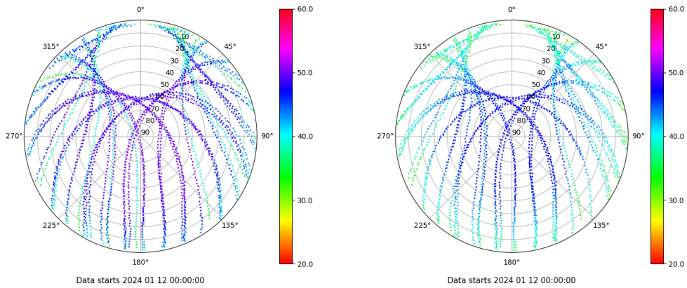
Skyplot for station RIO1. Signal to Noise S1C Data file RIO100ESP_R_2024012.xtr Skyplot for station RIO1. Signal to Noise S2P Data file RIO100ESP_R_2024012.xtr
