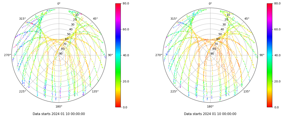
Skyplot for station RIO1. Parameter M1C Data file RIO100ESP_R_2024010.xtr Skyplot for station RIO1. Parameter M2P Data file RIO100ESP_R_2024010.xtr
