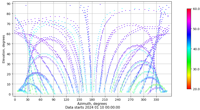
Azimuth-elevation plot for station RIO1. Signal to Noise S1C Data file RIO100ESP_R_2024010.xtr
