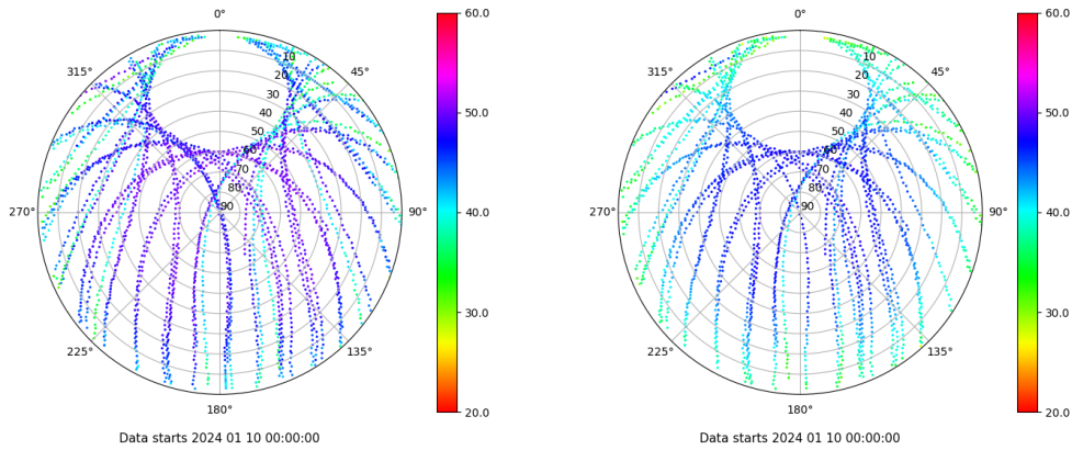
Skyplot for station RIO1. Signal to Noise S1C Data file RIO100ESP_R_2024010.xtr Skyplot for station RIO1. Signal to Noise S2P Data file RIO100ESP_R_2024010.xtr
