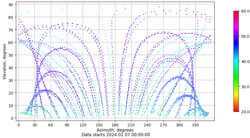
Azimuth-elevation plot for station RIO1. Signal to Noise S1C Data file RIO100ESP_R_2024007.xtr
