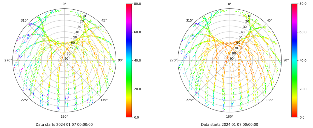
Skyplot for station RIO1. Parameter M1C Data file RIO100ESP_R_2024007.xtr Skyplot for station RIO1. Parameter M2P Data file RIO100ESP_R_2024007.xtr
