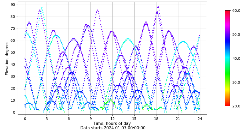
Time-elevation plot for station RIO1. Signal to Noise S1C Data file RIO100ESP_R_2024007.xtr
