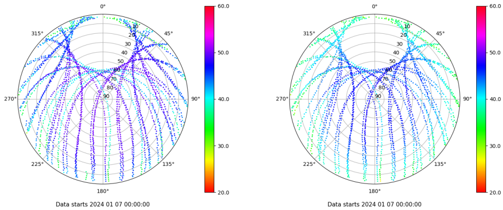
Skyplot for station RIO1. Signal to Noise S1C Data file RIO100ESP_R_2024007.xtr Skyplot for station RIO1. Signal to Noise S2P Data file RIO100ESP_R_2024007.xtr
