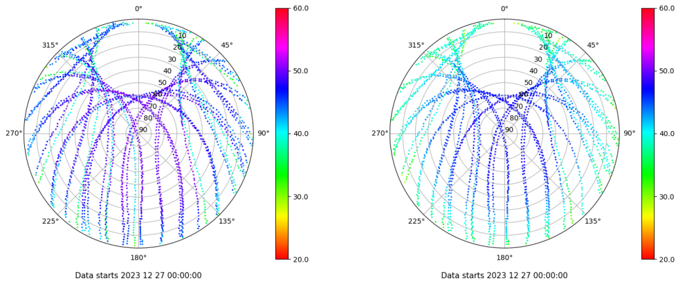
Skyplot for station RIO1. Signal to Noise S1C Data file RIO100ESP_R_2023361.xtr Skyplot for station RIO1. Signal to Noise S2P Data file RIO100ESP_R_2023361.xtr
