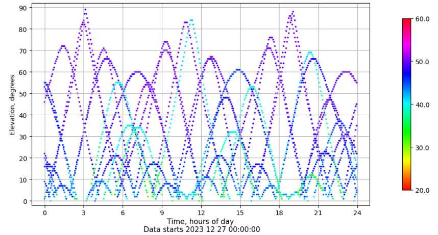
Time-elevation plot for station RIO1. Signal to Noise S1C Data file RIO100ESP_R_2023361.xtr
