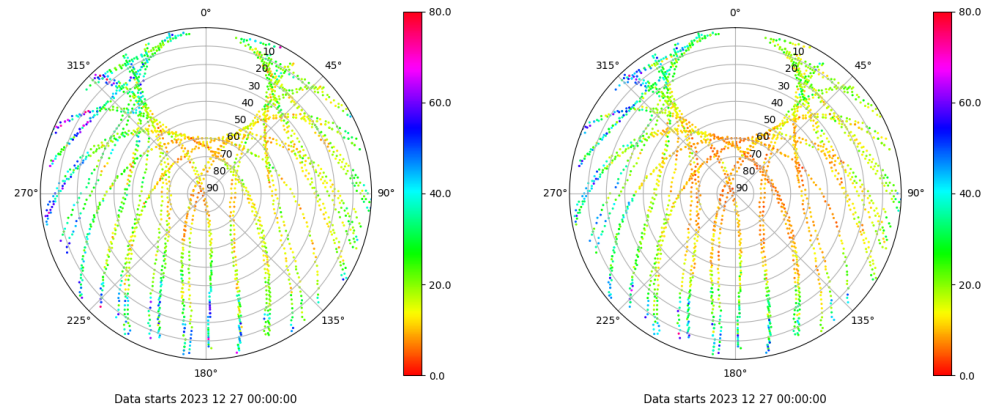
Skyplot for station RIO1. Parameter M1C Data file RIO100ESP_R_2023361.xtr Skyplot for station RIO1. Parameter M2P Data file RIO100ESP_R_2023361.xtr
