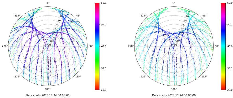
Skyplot for station RIO1. Signal to Noise S1C Data file RIO100ESP_R_2023358.xtr Skyplot for station RIO1. Signal to Noise S2P Data file RIO100ESP_R_2023358.xtr
