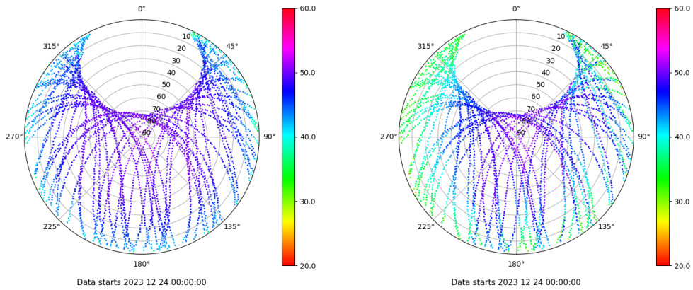
Skyplot for station RIO1. Signal to Noise S1C Data file RIO100ESP_R_2023358.xtr Skyplot for station RIO1. Signal to Noise S2W Data file RIO100ESP_R_2023358.xtr
