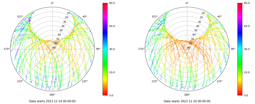
Skyplot for station RIO1. Parameter M1C Data file RIO100ESP_R_2023358.xtr Skyplot for station RIO1. Parameter M2W Data file RIO100ESP_R_2023358.xtr
