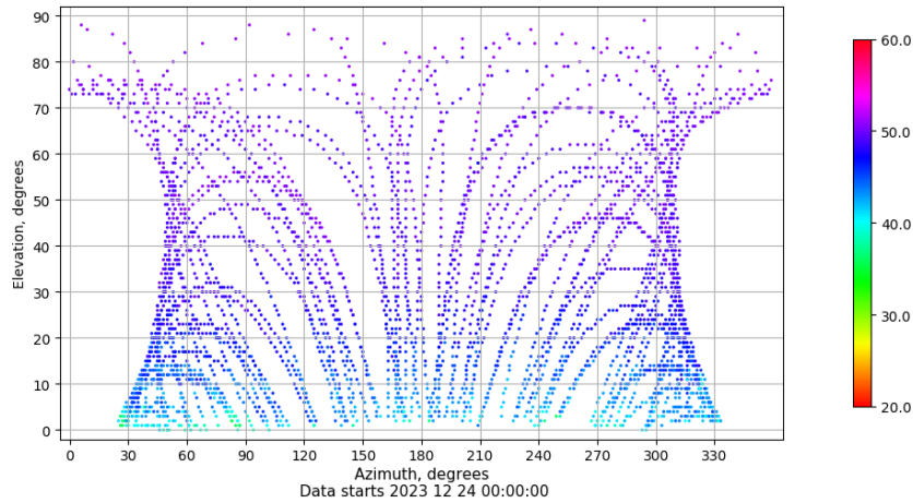
Azimuth-elevation plot for station RIO1. Signal to Noise S1C Data file RIO100ESP_R_2023358.xtr
