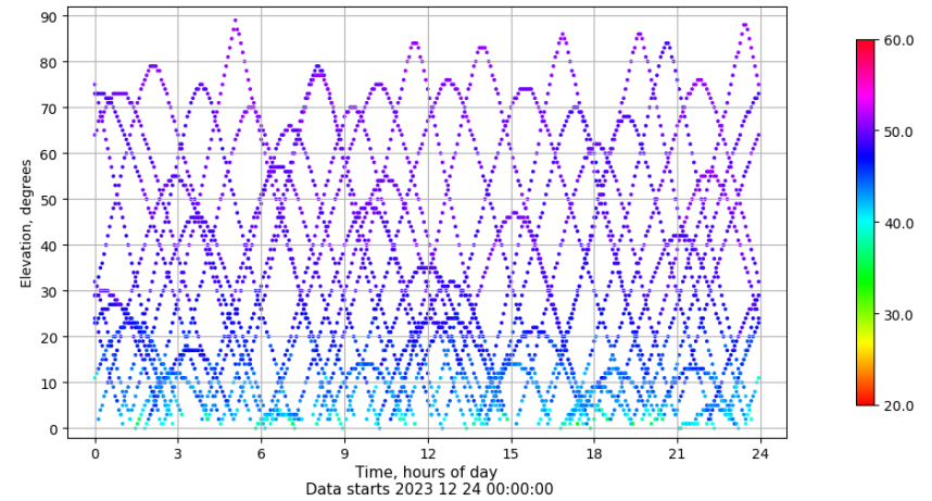
Time-elevation plot for station RIO1. Signal to Noise S1C Data file RIO100ESP_R_2023358.xtr
