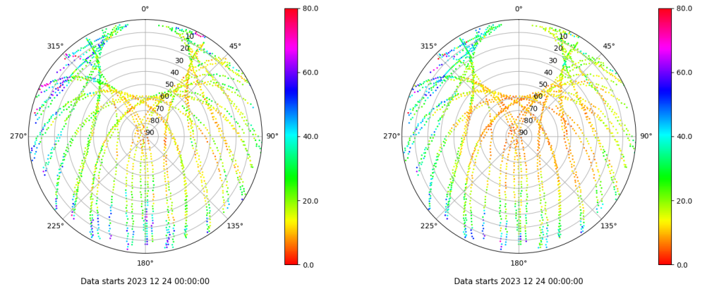
Skyplot for station RIO1. Parameter M1C Data file RIO100ESP_R_2023358.xtr Skyplot for station RIO1. Parameter M2P Data file RIO100ESP_R_2023358.xtr
